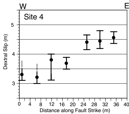
Figure 12. Variability of slip through the Kavak grove at site 4, showing mean values and uncertainties. Note the apparent systematic increase in slip from west to east.
