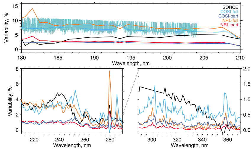
Figure 1. The relative difference (%) of the SSI between June 2004 and February 2009 for NRL-part, COSI-part, and SORCE data sets and the difference between solar maximum and minimum for NRL-full and COSI-full. All five data sets are plotted with a 1 nm sampling and are designated by colors given in the legend. The COSI-full data set is plotted, in addition, at a high resolution (light blue color). Different panels show different wavelength regions. Note the change of scale between the panels.
