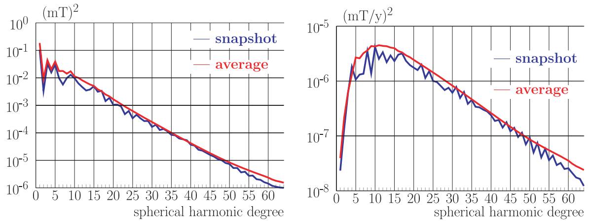
Figure 2. Mauersberger–Loves spectra at the core–mantle boundary for the field (left-hand panel) and the secular variation (right-hand panel) generated by the dynamo model (logarithmic scales), after application of the scaling procedure described in the text. In blue: instantaneous spectra for a randomly picked sample. In red: time-averaged spectra.
