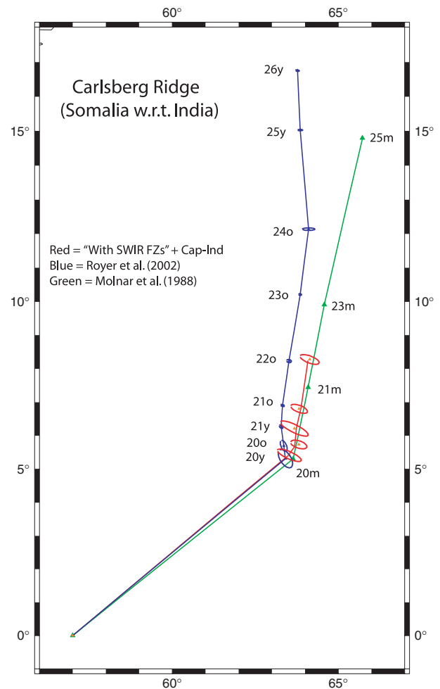
Figure 18. Trajectories of a point on the Somalia Plate relative to the Indian Plate for the three sets of Somali–India rotations in Fig. 17. Note that the trajectory based on the Royer et al. (2002) rotations lies about 60 km west of the trajectory based on the ‘With SWIR FZs’ rotations for anomalies 20o to 22o.
