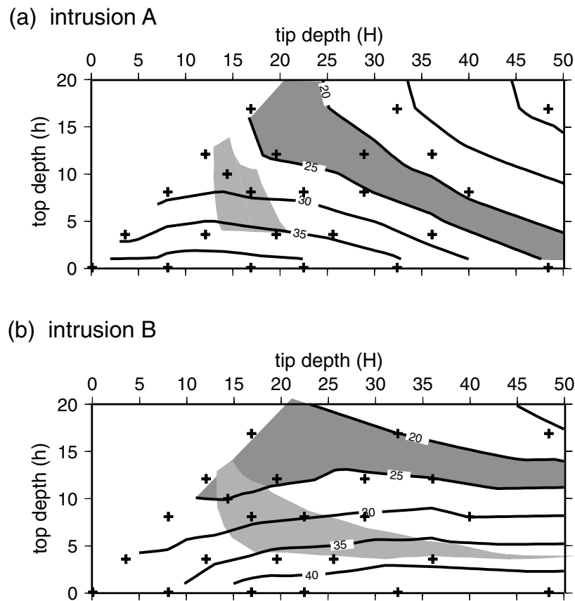
Figure 3. Determination of the 'best-fitting' parameters h and H , in the cases of intrusion shape A and B (see caption of Fig. 2 for their definition). Crosses show the couples ( h , H ) for which the geophysical outputs are calculated. The values of these outputs are interpolated within the range of investigated h and H . Thick lines represent the \Delta MBA between segment centres and segment ends. The lighter grey region represents the range of parameters h and H accounting for the observed maximal depths of the earthquakes. The darker grey region represents the range of parameters h and H accounting for the observed \Delta MBA amplitude.
