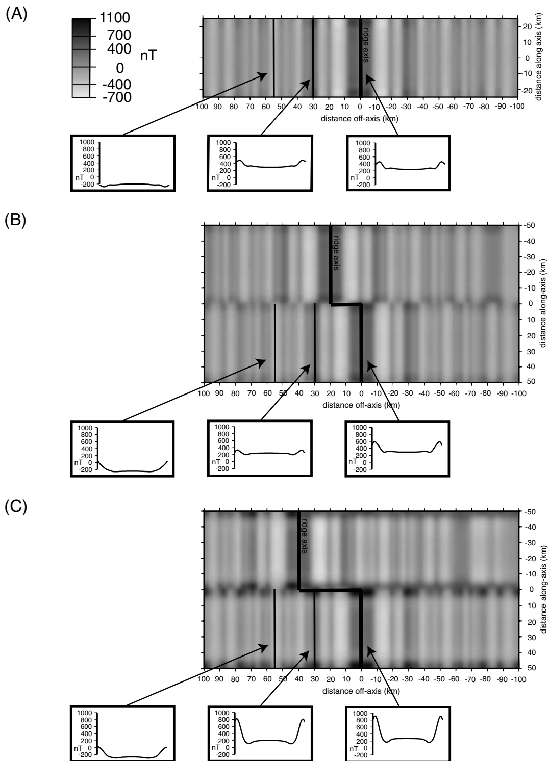
Figure 7. Modelled magnetic anomalies considering basalt (the Fe-Ti content variation is considered), gabbro and serpentinized peridotite magnetization (as shown along-axis on Fig. 5, D). (A) aligned segments; (B) 20 km offset segments and (C) 40 km offset segments. For each subset, top : modelled magnetic anomaly map; bottom : magnetic profiles along three isochrons. From left to right: sections along reversed chron 3r (5.5 Myr), normal chron 2A (3 Myr), and axis (0 Myr).
