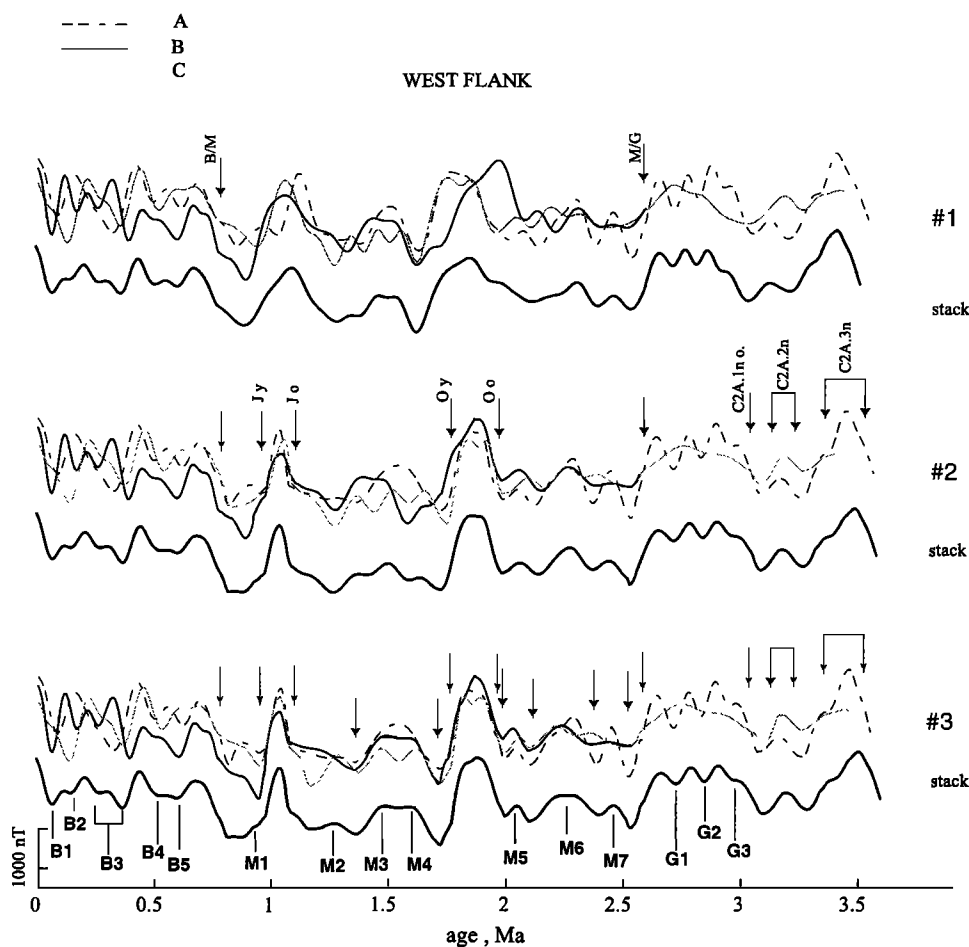
Figure 6b. Same as Figure 6a except for the western portions of the profiles.
