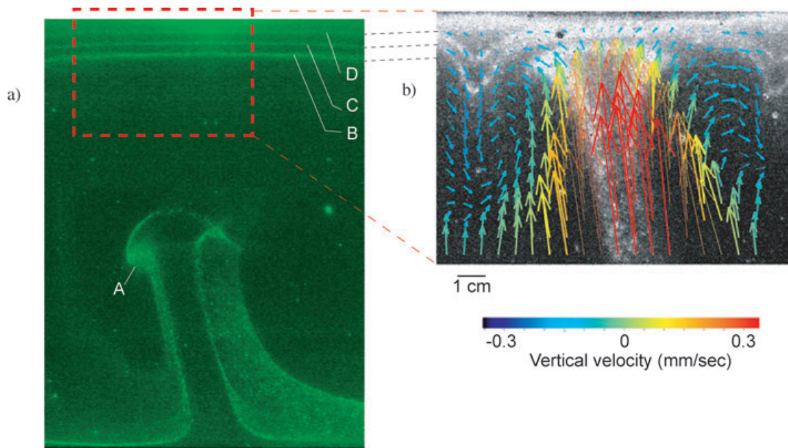
Figure 11. Experimental results: (a) A tank (30 × 30 cm; height 15 cm) of sugar syrup is cooled from above (at T = -16^\circ \text{C} ) and heated from below (at T = 52.4^\circ \text{C} ). The tank bulk interior is at temperature T_m = 36^\circ \text{C} . The viscosity ratio between the cold and the hot fluid is 3245, and the Rayleigh number, characterizing the intensity of convection, is 3.4 \times 10^6 , within mantle convection range. Bright white lines are isotherms ( A = 40.5^\circ \text{C} ; B = 31.4^\circ \text{C} ; C = 24.6^\circ \text{C} ; D = 10.4^\circ \text{C} ). A cold TBL below the upper surface is developing, while the bottom hot TBL has already become unstable and has generated a hot plume. The lateral dimension of the image is 10 cm. (b) Close up on the thermal (bright white lines) and velocity structures (coloured arrows) after the plume impact. The plume is surrounded by a ring of colder material and consequently the two bottom isotherms of the cold TBL (within the mobile part) are distorted.
