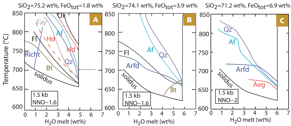
FIGURE 3 Phase relationships of peralkaline silicic magmas (NNO-1.6 and NNO-2 mean an f_{O_2} 1.6 or 2 log units below the NNO buffer, respectively). (A) and (B) Moderately peralkaline magma (comendite) from Kenya (Scaillet and Macdonald 2001; compositions 14 and 15 in TABLE 1, respectively). Horizontal dashed line in (A) is the H_2O -saturated solidus of the haplogranite system. (C) Strongly peralkaline magma (pantellerite) from Kenya (Scaillet and Macdonald 2006; composition 17 in TABLE 1). Phase abbreviations are as in FIGURES 1 and 2, plus Aeg (aegirine), Arfd (arfvedsonite), Fay (fayalite), Fl (fluorite), Hd (hedenbergite), Ox (oxides), Richt (richterite)
