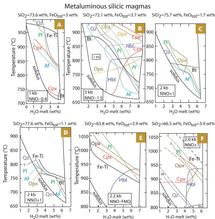
FIGURE 2 Phase relationships of metaluminous silicic magmas (NNO and FMQ are reference solid fO_2 buffers: NNO+1 means an fO_2 one log unit above NNO; NNO–FMQ means an fO_2 between those two buffers). (A) Fe-rich granite from Australia (Clemens et al. 1986; composition 7 in TABLE 1). (B) Fe-rich granite from NE Brazil (Dall'Agnol et al. 1999; composition 6 in TABLE 1). (C) and (D) Fe-poor granites from Australia (Klimm et al. 2008; compositions 12 and 13 in TABLE 1, respectively). Dashed lines on Brazilian granite (B) show the effect of increasing fO_2 up to NNO+2 on mineral stabilities. (E) Andesite from Mt. St. Helens (Rutherford et al. 1985; composition 10 in TABLE 1). (F) Dacite from San Pedro volcano (Costa et al. 2003; composition 11 in TABLE 1). Dotted lines on the dacite phase diagram give the melt fraction in wt%. Phase abbreviations are as in FIGURE 1 plus Cpx (clinopyroxene), Fe–Ti (Fe–Ti oxides), Hbl (hornblende), Ilm (ilmenite).
