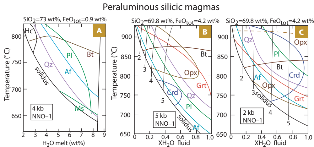
FIGURE 1 Isobaric T – H_2O_{melt} phase relationships of peraluminous silicic magmas (NNO–1 means an fO_2 one log unit below the NNO solid buffer). (A) Fe-poor leucogranite from the High Himalayas (composition 4 in TABLE 1; Scaillet et al. 1995). (B) and (C) Fe-rich granite from SE Australia (Clemens and Birch 2012; composition 2 in TABLE 1). In (B) and (C) , the H_2O_{melt} is shown as isopleths labeled as 2, 3, 4 and 5. The black near-vertical curve at high H_2O_{melt} in (A) is the water solubility curve. The black curve on
