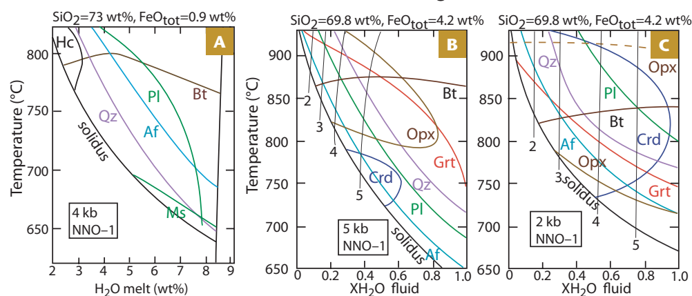
FIGURE 1 Isobaric T – H_2O_{\text{melt}} phase relationships of peraluminous silicic magmas (NNO–1 means an fO_2 one log unit below the NNO solid buffer). (A) Fe-poor leucogranite from the High Himalayas (composition 4 in TABLE 1; Scaillet et al. 1995). (B) and (C) Fe-rich granite from SE Australia (Clemens and Birch 2012; composition 2 in TABLE 1). In (B) and (C), the H_2O_{\text{melt}} is shown as isopleths labeled as 2, 3, 4 and 5. The black near-vertical curve at high H_2O_{\text{melt}} in (A) is the water solubility curve. The black curve on
