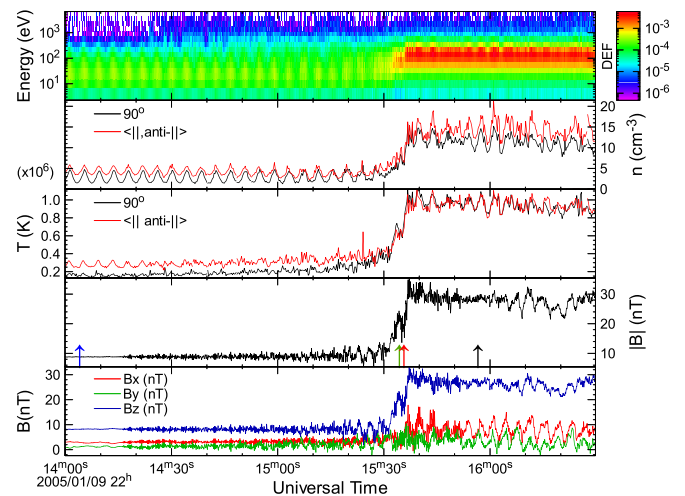
FIG. 2 (color online). Overview of data from Cluster 2 on 9 Jan. 2005. From top to bottom: Omni-directional electron energy-time spectrogram @250 ms resolution, electron pseudodensity, electron pseudotemperatures (see Method), magnetic field magnitude, and field components. Arrows in the fourth panel show locations of the cuts presented in Fig. 4.
