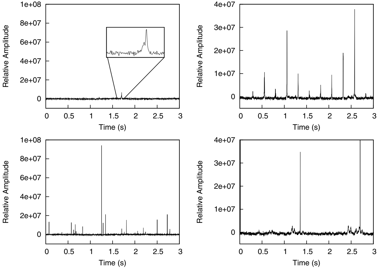
Fig. 18. Observations of PSR B0950+08 made using the LBAs (left) and HBAs (right). The top panels show sections of the timeseries after dedispersion to the pulsar DM of 2.96 \text{ pc cm}^{-3} . We easily detect single pulses and one can see the wide range in intensity of the pulses, in particular in the low band. In the lower panels the same timeseries are shown but without dedispersion, the so-called DM zero timeseries. In both the LBAs and HBAs we can see evidence for narrow spikes of RFI at zero DM, however these are clearly broadband in nature and have been completely dispersed beyond a detectable level at the dispersion measure of the pulsar. We note that the broad features seen in the DM zero timeseries of the HBAs (e.g. near 2.5 s in the lower-right panel) are due to the pulsar itself. The ordinate axes corresponds to an arbitrary amplitude but is preserved in the top and bottom plots.
