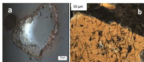
Fig. 2: a -Flaking of quartz in arkoses from Chaillac; b- quartz from Rochechouart stockwork with two fracture sets parallel to the rhomboedra
