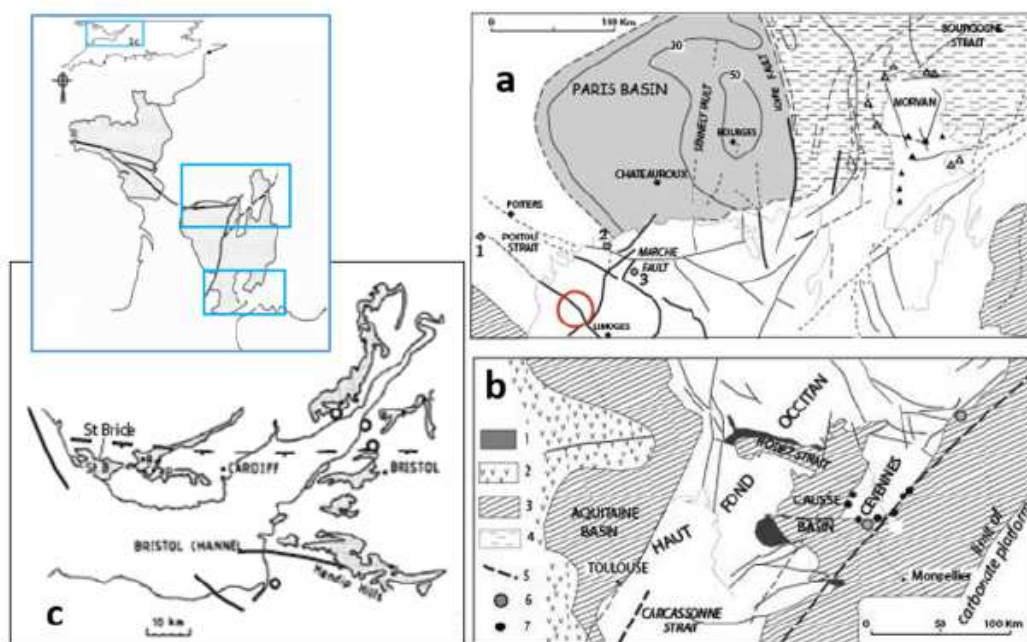
Fig. 1. Distribution of stratabound and vein F Ba Pb Fe Mn ores on the LH paleosurface close to north and south FMC basement rocks (Fig. 1a and 1b, respectively, modified after Blès et al. 1989), and Mn ores from the Bristol-Mendip area (Fig. 1c, modified after Evans and Kermak 1997). The relative position of the 3 selected areas is given in inset. Legend of figures 1a and 1b: 1= Permian; 2= evaporites; 3= carbonate platform; 4= marls. 5= flexure. Selected ores in Fig. 1a: 1=Pb Ag mine of Melle; 2=vein and stratabound Ba F Fe Mn ores from Chaillac; 3= Fanay U mine; triangles = stratabound (empty symbols) and vein fluorite (full symbols) from Morvan. Black star: iron mines from Burgundy. White star: ochres from Auxerre region. The large circle represents the Rochechouart crater. Fig. 1b: 6= Pb Zn mines (Largentière to the north and Les Malines to the south) and showings (= 7) from the Cévennes margin, after Macquar et al. (1990). Empty dots in Fig. 1c are outcropping deformed soft sediments after Simms (2003). See text for reference
