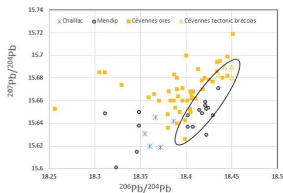
Fig. 3 : ^{207}\text{Pb}/^{204}\text{Pb} versus ^{206}\text{Pb}/^{204}\text{Pb} isotopic ratios of various mineralizations linked to the Hettangian paleosurface in WE. Data sources: Marcoux (1987, Chaillac), Haggerty et al. (1996, Mendip Hills), Le Guen et al (1991; Cévennes). Ellipse: galena and slag field from Melle after Téreygeol et al (2004)
