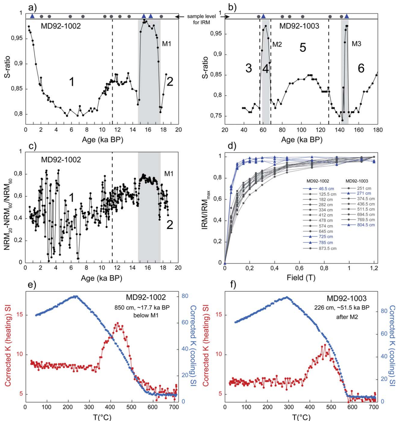
Figure 5. (a and b) S ratio for cores MD92–1002 and MD92–1003. The high values correspond to the M1–M3 episodes. (c) R ratio ((NRM 20 mT – NRM 60 mT )/NRM 60 mT ). (d) IRM acquisition curves for cores MD92–1002 and MD92–1003. Rapid saturation is obtained for samples within the peaks (blue curves). (e and f) Thermomagnetic curves of two samples from cores MD92–1002 and MD92–1003 outside the M1 and M2 susceptibility peaks.
