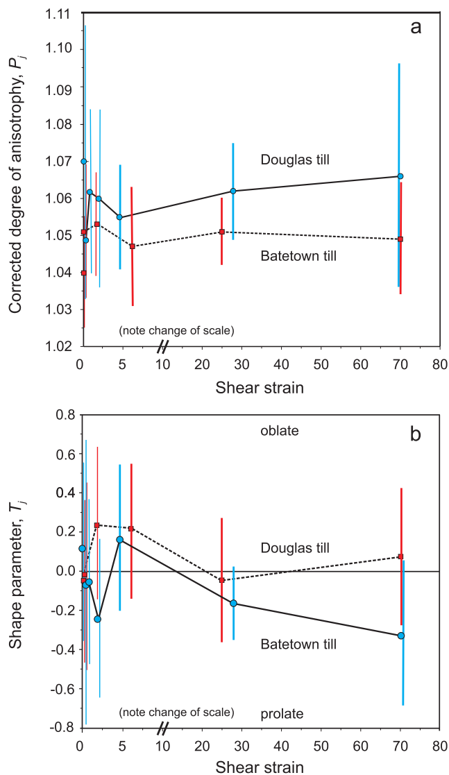
Figure 7. (a) Corrected degree of anisotropy and (b) shape parameter as a function of shear strain for the Batetown and Douglas tills. Error bars indicate \pm 1 standard deviation.
