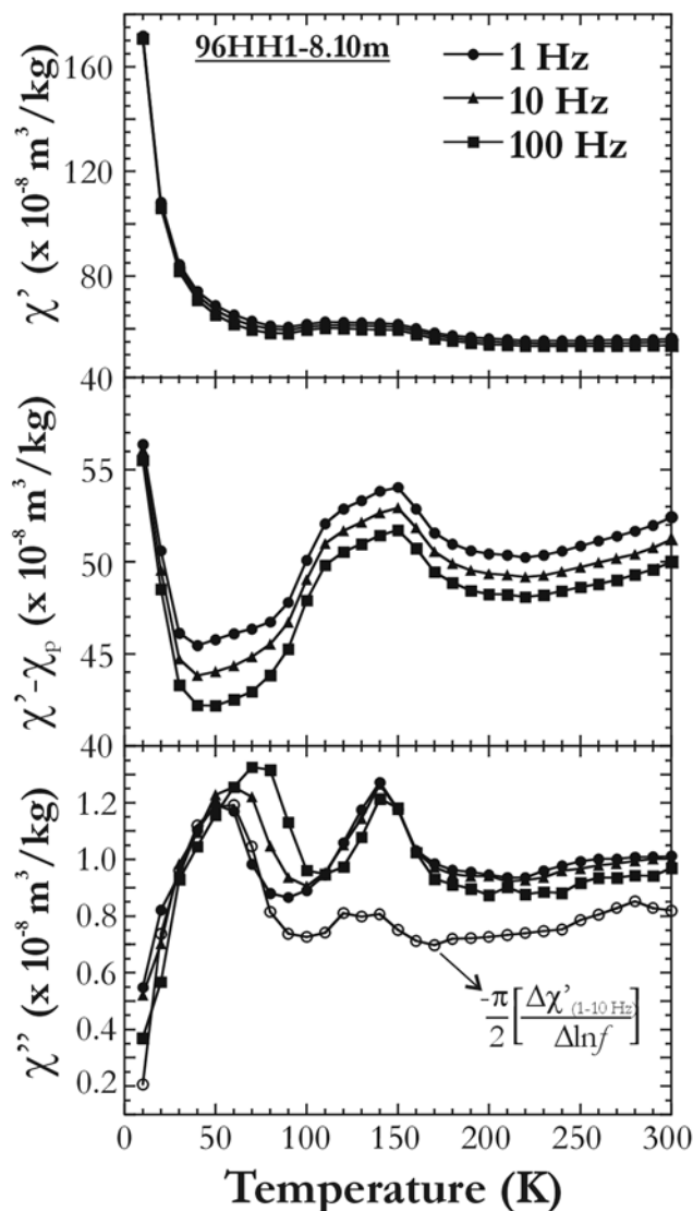
Figure 11. (top) In-phase and (bottom) quadrature components of magnetic susceptibility measured between 10 K and 300K in a constant 240 A/m field amplitude and at seven frequencies (1, 3, 10, 30, 100, 300, and 1000 Hz; not all shown) for sample 96HH1-8.10m. (middle) Paramagnetic component subtracted from the in-phase susceptibility in order accentuate the variability due only to the 90% Ti ilmenite-hematite series phase present in low concentration in the sample.
