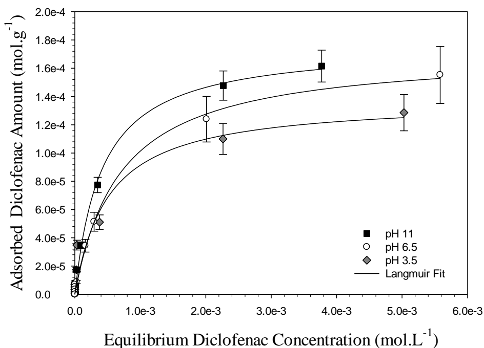
Fig. 7. Equilibrium adsorption isotherms of diclofenac ( pK_a=4.51 ) onto HDTMA-Mt organoclay (prepared at a concentration of 4 times the CEC of the starting Mt) for three different pH values of 3.5, 6.0-6.5, and 11.0. The efficiency of the adsorption is enhanced at high pH.
