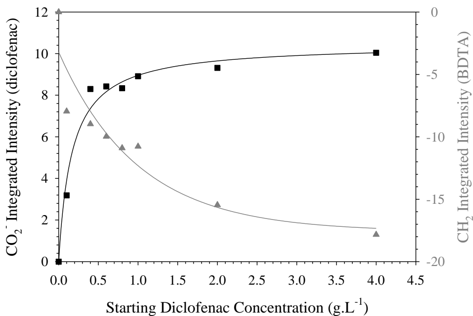
Fig. 4. Evolution of normalized integrated FTIR intensity of both CO 2 - bands (diclofenac) and CH 2 bands (surfactants) as a function of the starting diclofenac concentration. The lines are guides for the eyes.
