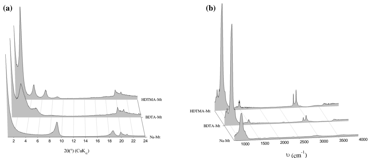
Fig. 1. (a) XRD patterns for dehydrated Na-Mt, BDTA-Mt and HDTMA-Mt organoclays. (b) FTIR spectra of Na-Mt, BDTA-Mt and HDTMA-Mt organoclays. The proper intercalation of both surfactants is confirmed by the shift of the first 00l reflection at low angle values (XRD data) and with the \text{CH}_2 scissoring and stretching bands of the alkyl tails of the organic cations.
