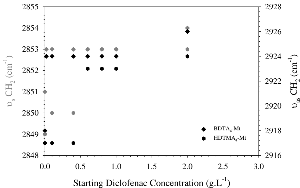
Fig. 5. Representation of the change in frequency of the symmetric and asymmetric CH 2 stretching bands of the HDTMA-Mt and BDTA-Mt organoclays as a function of the starting diclofenac concentration.
