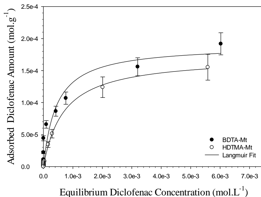
Fig. 2. Effect of the chemical nature of cationic surfactant (BDTA-Mt and HDTMA-Mt) on adsorption of diclofenac at ambient temperature (25°C) and using starting concentration of diclofenac ranging from 10 mg L -1 to 2 g L -1 .
