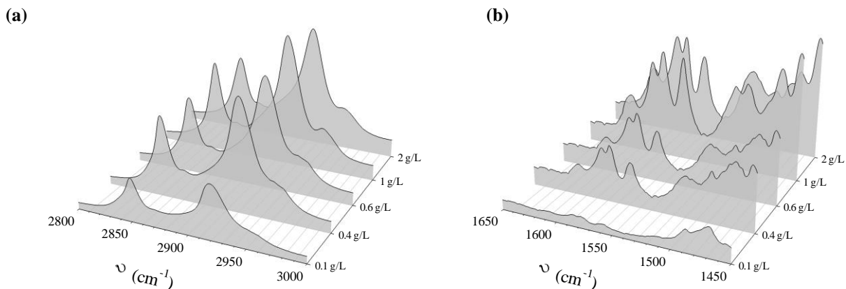
Fig. 3. 3D evolution of the FTIR spectra in the wavenumbers window of CH 2 stretching bands for (a) HDTMA-Mt organoclay in the range 2800-3000 cm -1 and the (b) CO 2 - stretching bands of diclofenac in the range 1450-1650 cm -1 for different starting diclofenac concentrations (0.1, 0.4, 0.6, 1 and 2 g L -1 ).
