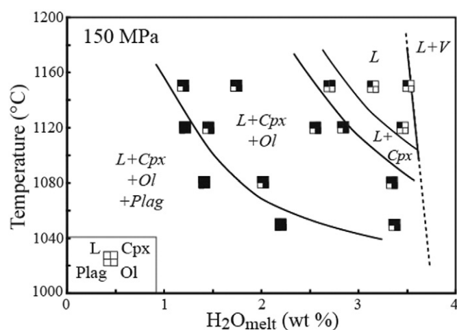
Fig. 6. Experimentally determined T- H_2O_{\text{melt}} phase diagram for Som-1 at P = 150 MPa. Experimental data in Table 2. Squares give conditions of experimental charges and types of phase assemblages encountered. Open square: phase is absent; filled square: phase is present. Note that Fe-oxide occurs in most charges although its presence could not be confirmed in all because of its small size. L: liquid; Cpx: clinopyroxene; Ol: olivine; Plag: plagioclase. All charges include a fluid phase (see text). Pure H_2O vapour is designated as V and the L - L + V phase boundary is the H_2O solubility curve.
