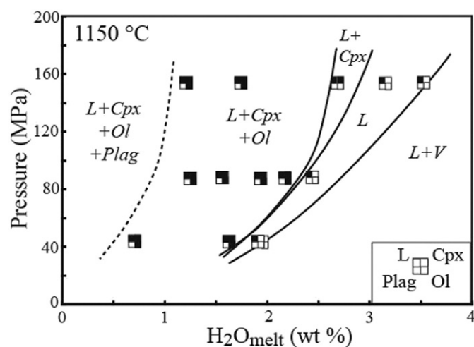
Fig. 7. Experimentally determined P- H_2O_{\text{melt}} phase diagram for Som-1 at T = 1150 °C. Experimental data in Table 2. Squares give conditions of experimental charges and types of phase assemblages encountered. Open square: phase is absent; filled square: phase is present. Note that Fe-oxide occurs in most charges although its presence could not be confirmed in all because of its small size. L: liquid; Cpx: clinopyroxene; Ol: olivine; Plag: plagioclase. All charges include a fluid phase (see text). Pure H_2O vapour is designated as V and the L - L + V phase boundary is the H_2O solubility curve. The location of the plagioclase saturation curve (dashed) is estimated.
