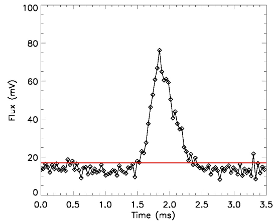
Figure 3. Example of the output voltage recorded by the 12^\circ channel photodiode for ambient air particles crossing the laser beam. The red line corresponds to the threshold for the peak detection. When a particle is detected, the signal must return back below the threshold to allow the detection of the next one.
