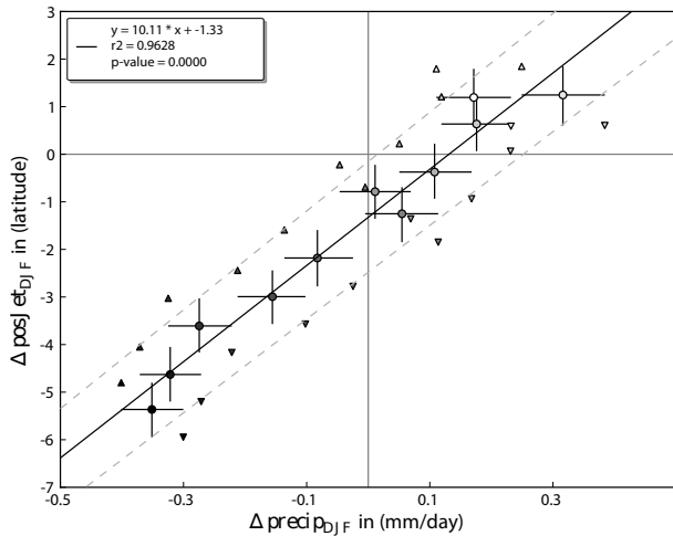
Figure 10. 850 hPa winter jet-stream shift (in latitude) vs. winter precipitation anomaly over the Scandinavian region. The range of results has been obtained by bootstrapping. Up and down triangles represent the 5th precipitation percentile vs. the 95th jet position percentile, and the 95th precipitation percentile vs. the 5th jet position percentile respectively. Circles are the average values and crosses indicate the 5th and 95th percentiles.
