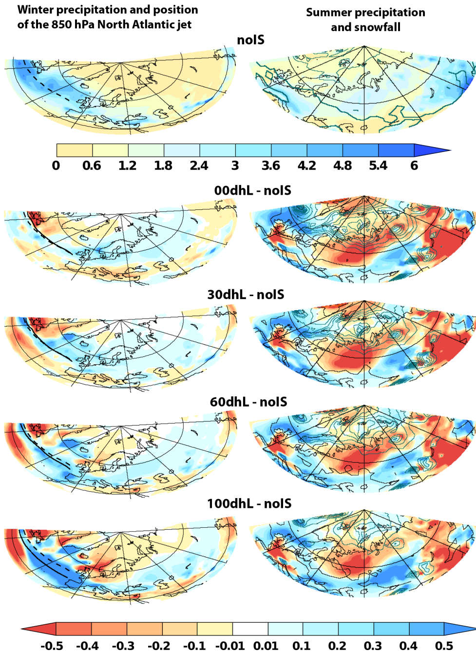
Figure 9. (shaded) and position of the North Atlantic jet stream without LIS (dashed) and for the x xdhL experiment (solid line). Right column: summer precipitation (shaded) and snowfall (contour every 0.1 \text{ mm day}^{-1} , blue contour for positive values).
