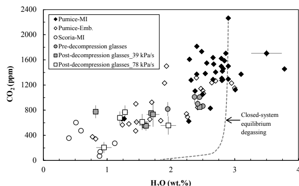
FIGURE 8. \text{H}_2\text{O} and \text{CO}_2 contents in natural glasses from Stromboli (data from Métrich et al. 2010) and comparison with experimental series #2 glasses from this study (39 kPa/s, Table 5) and from Le Gall and Pichavant (2016, 78 kPa/s). Stromboli glasses plotted include melt inclusions (MI) and embayments (Emb.) from pumices and scoriae. Experimental glasses include pre- (circles) and post-decompression glasses (squares). The closed system equilibrium degassing trend (dashed curve) is calculated using VolatileCalc (Newman and Lowenstern 2002).
