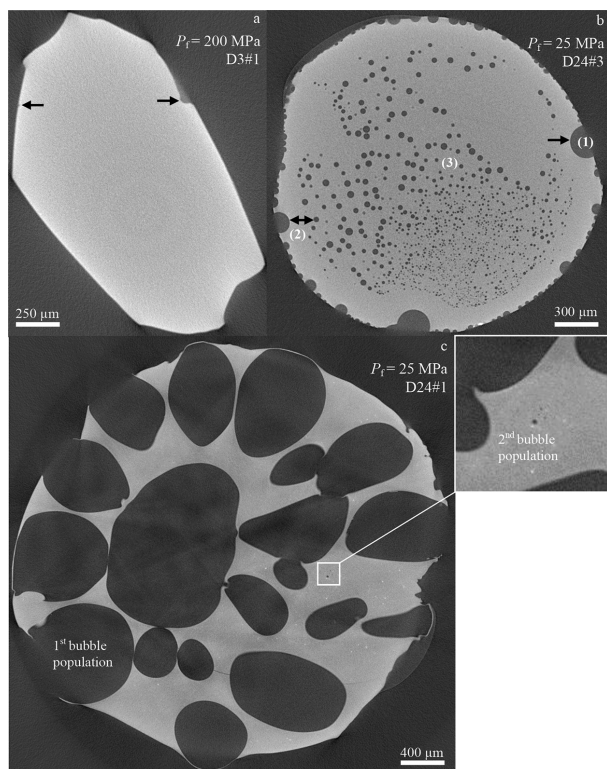
FIGURE 1. Representative types of textures of post-decompression glass samples. (a) Tomographic slice of sample D3#1 quenched at P_t = P_m = 200 MPa, showing a bubble-free core and a thin (<50 µm) bubbly rim indicated by black arrows. (b) Tomographic slice of sample D24#3 decompressed to 25 MPa P_t , showing three distinct zones: (1) a thick (150–200 µm) bubbly rim indicated by a black arrow, (2) a bubble-free zone depleted in volatiles delimited by a double black arrow, and (3) a core with numerous nearly homogeneously distributed bubbles. (c) Tomographic slice of sample D24#1 decompressed to 25 MPa P_t , characterized by two distinct bubble populations. The inset gives a close-up view of the small bubbles that correspond to the second bubble population. See Table 3 for details about the experimental conditions and textural results.
