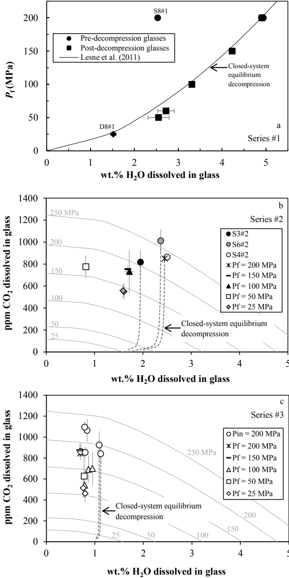
FIGURE 5. H 2 O and CO 2 concentrations in pre- and post-decompression glasses. (a) Plot of series #1 H 2 O concentrations as a function of final pressure P_f . H 2 O solubilities are computed using the Lesne et al. (2011b) regression equation. They define the closed-system equilibrium decompression path (black continuous line). H 2 O vs. CO 2 concentrations in series #2 and #3 glasses are shown in b and c, respectively. Circles = pre-decompression glasses synthesized at 200 MPa P_i (initial pressure); crosses = glasses decompressed to 200 MPa P_f (final pressure); rectangles = glasses decompressed to 150 MPa P_f ; triangles = glasses decompressed to 100 MPa P_f ; squares = glasses decompressed to 50 MPa P_f ; diamonds = glasses decompressed to 25 MPa P_f . In b, the symbol color refers to the synthesis experiments, either S3 (black), S6 (gray), or S4 (white, Table 2). Error bars (standard deviations, Table 5) are indicated on the data points. The thin continuous lines are fluid-melt equilibrium saturation isobars (25–250 MPa) and the dashed curves are equilibrium decompression paths calculated for some series #2 and #3 glasses assuming closed-system behavior. Equilibrium fluid-melt calculations were performed with VolatileCalc (Newman and Lowenstern 2002).
