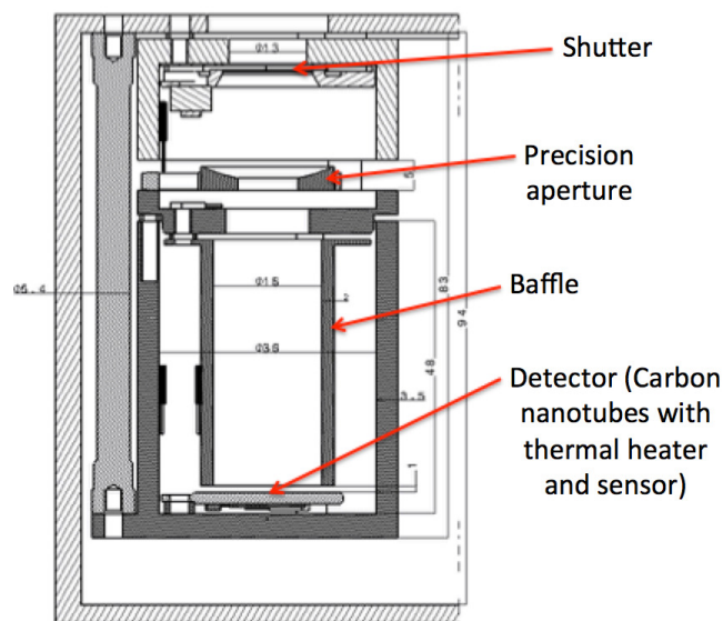
Figure 7. Main design of the SERB solar radiometer.
