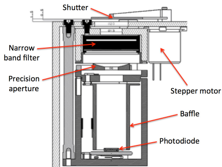
Figure 8. Main design of the SERB solar photometer.
