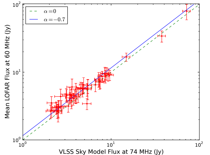
Figure 6. Plot of the mean extracted flux of sources from the 297 minutes NCP survey at 60 MHz against the cross-matched VLSS survey at 74 MHz. The solid line represents the expected LOFAR flux density assuming a spectral index of \alpha = -0.7 . For illustrative purposes a dashed-line representing \alpha = 0 (a 1:1 ratio) is also shown.
