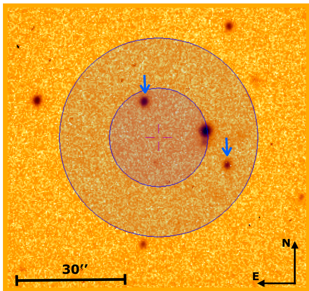
Figure 14. The resultant combined optical image obtained with follow-up observations using the Liverpool Telescope. It reaches a depth of r' \sim 22\text{--}22.5 mag and is calibrated against the USNO-B1 catalogue (Monet et al. 2003). The inner circle marked on the image, centred at the reported LOFAR transient position, represents a 1\sigma positional error of radius 14 arcsec. The outer circle shows the 2\sigma positional error circle of radius 28 arcsec. The two stars which have proper motions higher than 100 \text{ mas year}^{-1} , as indicated by the USNO-B1 (Monet et al. 2003) catalogue, are indicated by arrows.
