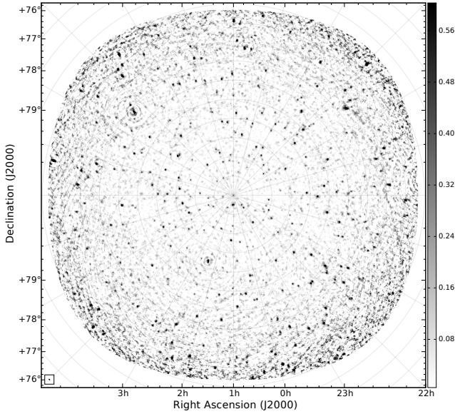
Figure 7. The deepest map produced of the NCP field from the survey. It was constructed by averaging all 31 of the 297-minute-duration images together in the image plane, using inverse-variance weighting. It has a noise level of 71 \text{ mJy beam}^{-1} and a resolution of 3.1 \times 1.4 \text{ arcmin} (BPA 42^\circ ). A total of 150 sources are detected at a 10\sigma level within a radius of 7.5 \text{ deg} from the centre of the map. While none of these sources are previously undetected, it provided a detailed reference map to check any transient candidates. The colour bar units are \text{Jy beam}^{-1} .
