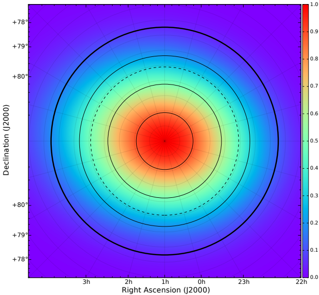
Figure 4. An example of a normalized primary beam map from one of the NCP observations, which has been scaled to 1.0. The bold, outer solid-line circle represents the full extent of the area for which the transient search was performed (radius of 7.5 deg). The inner solid-line circles show how the area was divided in order to gain an estimate of the average rms for each image accounting for the primary beam. The dashed-line circle indicates the position of the primary beam half-power point.
