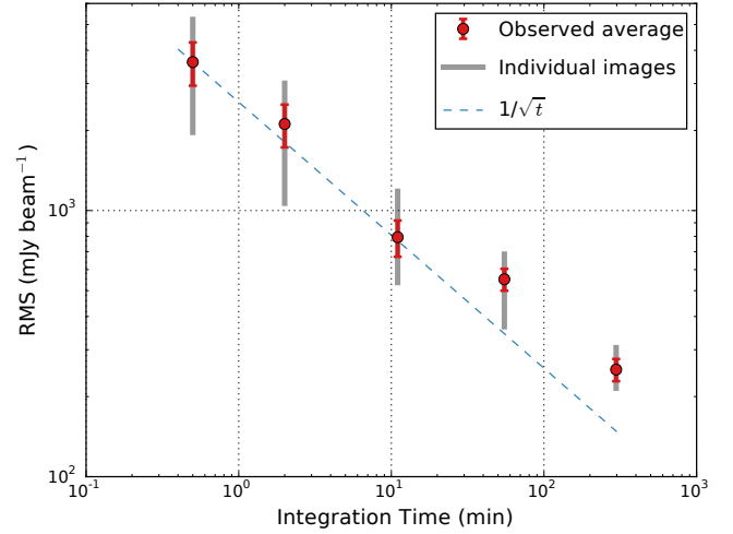
Figure 5. The average rms obtained from the images produced by combining and splitting the dataset. Also plotted in light grey are the range of noise values for the individual images at their respective time-scales, in addition to the 1/\sqrt{t} relation where t is the integration time of the observation. It can be seen that the average rms values approximately follow this relation; the longer time-scale values are likely to be slightly overestimated due to the methods used to estimate the rms. The errors shown on the average points are one standard deviation of the rms measurements from the respective time-scale.
