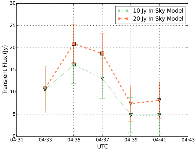
Figure 12. The extracted flux of the transient candidate in 2-minute intervals, obtained using the TRAP, for the cases where the transient is included in the sky model at 10 and 20 Jy. Data points represented by a square signify that the source was extracted from the image with a blind detection. In contrast, the triangles represent flux values obtained from a forced fit at the source position, where the source was no longer above the source extraction threshold (13 Jy, 5\sigma ). The two light curves follow the same trend, suggesting that the transient is brighter than a 3\sigma limit of 7.5 Jy in the 4-minute period of 04:34 - 04:38. The 10-Jy input case, returning a measured flux of 16 Jy, also suggests that 16 Jy may be the correct flux during this time frame. These light curves were obtained by extending the phase-calibration time interval to one min. The date of the observation was 2011 December 24.
