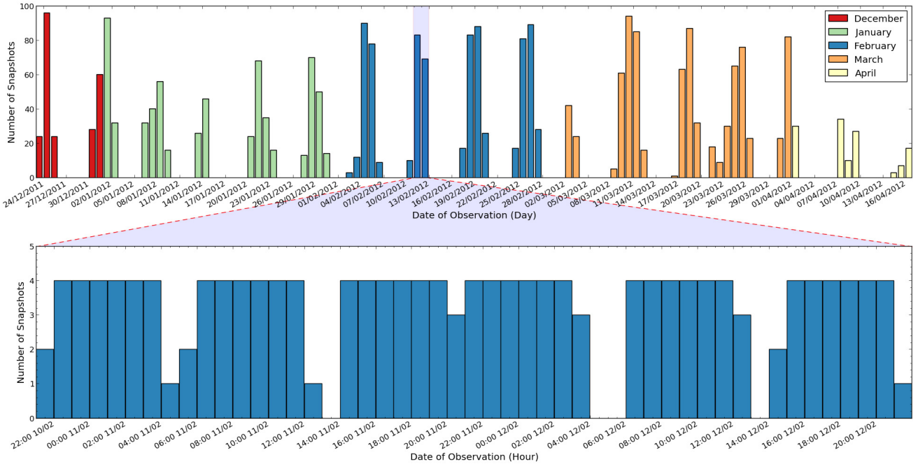
Figure 1. Histograms giving a general overview of when the 2609 11-minute snapshots of the NCP were observed. The top panel contains a histogram showing how many snapshots were observed on each day over the entire four month period, colour coded by month, which shows the distinct observing blocks in which NCP observations were obtained. The bottom panel displays a ‘zoom-in’ of the date range 21:00 2012/02/10–21:00 2012/02/12 UTC, now showing the number of snapshots per hour. This emphasises further the sometimes fragmented nature of the observing pattern of the NCP, with which careful consideration had to be given on how to combine the observations for the transient search.
