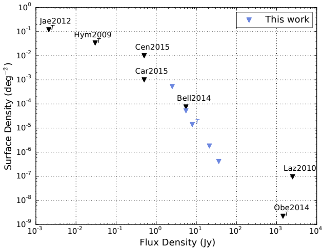
Figure 15. The logarithm of the surface density (deg ^{-2} ) against the logarithm of the flux density (Jy) of low-frequency transient surveys. We do not consider variable source limits. The surface densities for which transients have been detected are marked with a T . The surveys included are as follows: Hyman et al. (2005, 2006, 2009) (Hym2009); Lazio et al. (2010) (Laz2010); Jaeger et al. (2012) (Jae2012); Bell et al. (2014) (Bel2014); Obenberger et al. (2014a) (Obe2014); Carbone et al. (2015) (Car2015) and Cendes et al. (2015) (Cen2015).
