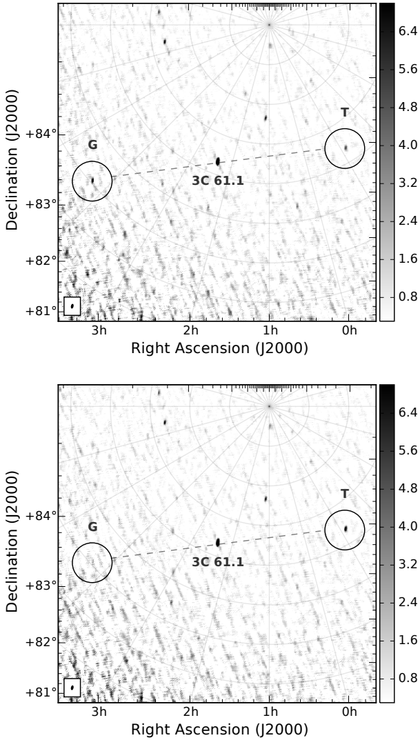
Figure 9. Upper Panel: Illustrates how the transient source (labelled ‘T’), ILT J225347+862146, was originally detected in the image, along with the associated ghost source (labelled ‘G’) across from 3C 61.1. Lower Panel: Now the measurement set as been re-calibrated with the transient included in the sky model; the ghost source has vanished. Upon closer inspection, other faint, source-like features also disappear from the re-calibrated image. These are most likely fainter ghost features which are reduced when the data were calibrated with a more complete sky model. The colour bar units are \text{Jy beam}^{-1} .
