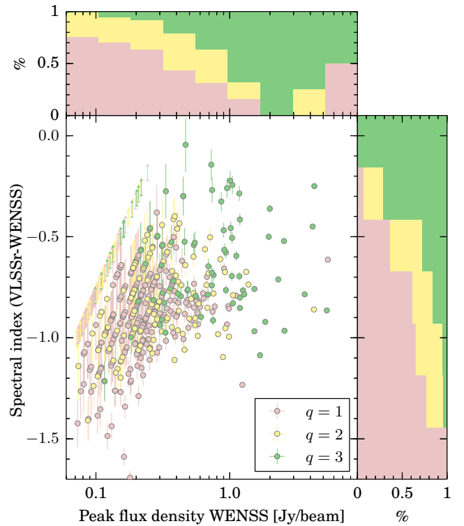
Fig. 7. Source quality as a function of low-frequency spectral index and WENSS peak flux density. Red, yellow, and green colours represent q = 1, 2 , and 3 , respectively. q = 3 corresponds to suitable primary calibrators. The histograms show the percentage of sources at each quality value. The histogram on the right does not include the sources with upper limits in their spectral indexes. The uncertainties of some of the values are smaller than the symbols, especially for the WENSS peak flux density. The stripes at low peak flux densities are due to sources detected at multiples of the rms noise of VLSSr.
