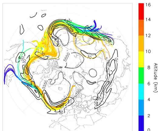
Figure 6. Ten day backward trajectories for a cluster centered at 11130 m on 7 August 2009 coupled with the ERA-Interim horizontal wind module (m/s) (solid line) at 200 hPa and geopotential height (m) (dashed-dotted line) at 500 hPa on 29 July 2009.
