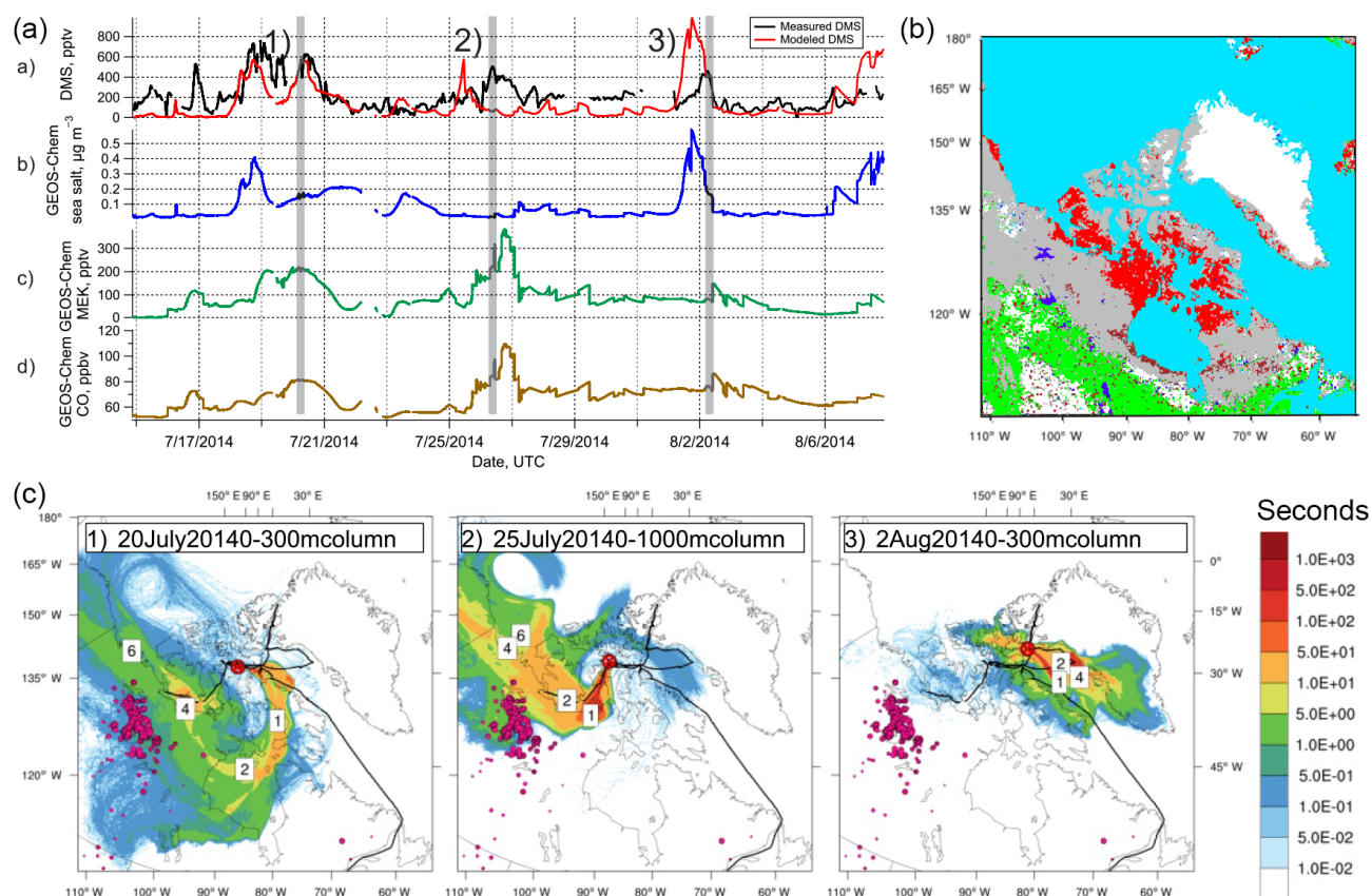
Figure 3. (a) Surface-layer atmospheric time series along Amundsen ship track of (a) measured and GEOS-Chem (GC) simulated DMS; (b) GC simulation of accumulation mode sea salt mass concentration; (c) GC simulation of methyl ethyl ketone (MEK) mixing ratio; (d) GC simulation of carbon monoxide (CO) mixing ratio. (b) Olson Land Cover map of North America showing low-lying tundra (red), other tundra (grey), forest (green), wetlands and marsh (brown), and inland water (dark blue). (c) FLEXPART-WRF potential emissions sensitivity (PES) simulation plots showing the likely origin of the air mass at the ship position. The colour scale in seconds corresponds to time spent in the lower 300–1000 m (marked on each plot) before arriving at the ship position. The three plots correspond to the three periods shown by the numbers and shaded bars in (a), showing examples of (1) transport from lower latitudes, including Hudson Bay (2) continentally influenced air (3) local marine influence from Baffin Bay.
