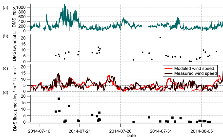
Figure 2. Time series along Amundsen ship track of (a) atmospheric DMS mixing ratio (10 Hz) from HR-ToF-CIMS, (b) observed DMS surface seawater concentration, (c) hourly-averaged wind speed at ship position (black) and hourly-average GEOS wind speed at ship position (red), and (d) DMS water-air flux estimates.
