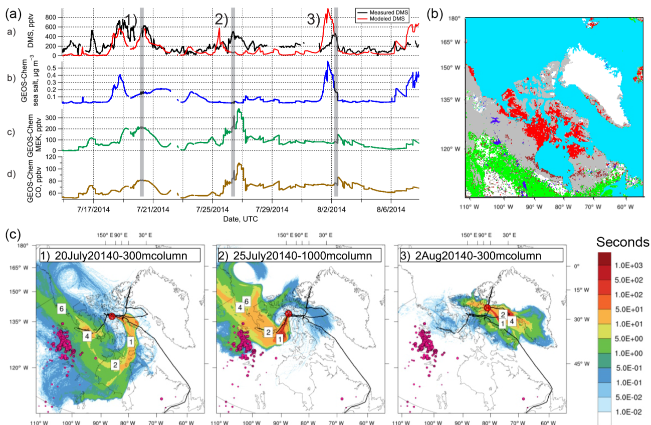
Figure 3. (a) Surface-layer atmospheric time series along Amundsen ship track of (a) measured and GEOS-Chem (GC) simulated DMS; (b) GC simulation of accumulation mode sea salt mass concentration; (c) GC simulation of methyl ethyl ketone (MEK) mixing ratio; (d) GC simulation of carbon monoxide (CO) mixing ratio. (b) Olson Land Cover map of North America showing low-lying tundra (red), other tundra (grey), forest (green), wetlands and marsh (brown), and inland water (dark blue). (c) FLEXPART-WRF potential emissions sensitivity (PES) simulation plots showing the likely origin of the air mass at the ship position. The colour scale in seconds corresponds to time spent in the lower 300–1000 m (marked on each plot) before arriving at the ship position. The three plots correspond to the three periods shown by the numbers and shaded bars in (a), showing examples of (1) transport from lower latitudes, including Hudson Bay (2) continentally influenced air (3) local marine influence from Baffin Bay.
