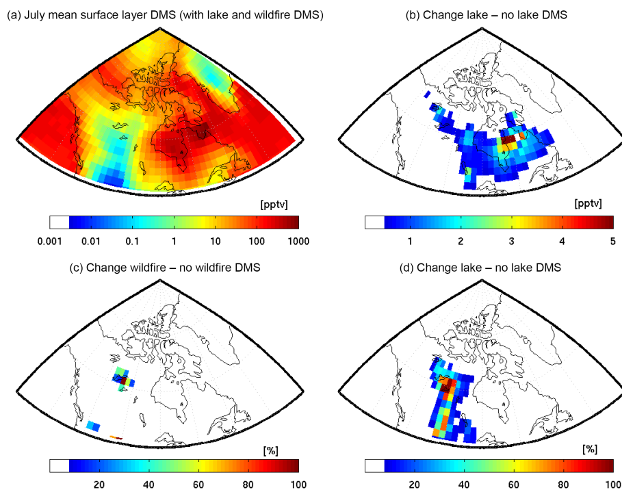
Figure 5. (a) GEOS-Chem simulated July mean surface-layer atmospheric DMS in Canada; (b) absolute change in simulated surface-layer DMS with implementation of lake DMS emissions; (c) percent change in simulated Canadian surface-layer DMS due to DMS emissions from wildfires; (d) percent changes in simulated surface-layer DMS with the implementation of lake DMS emissions.
