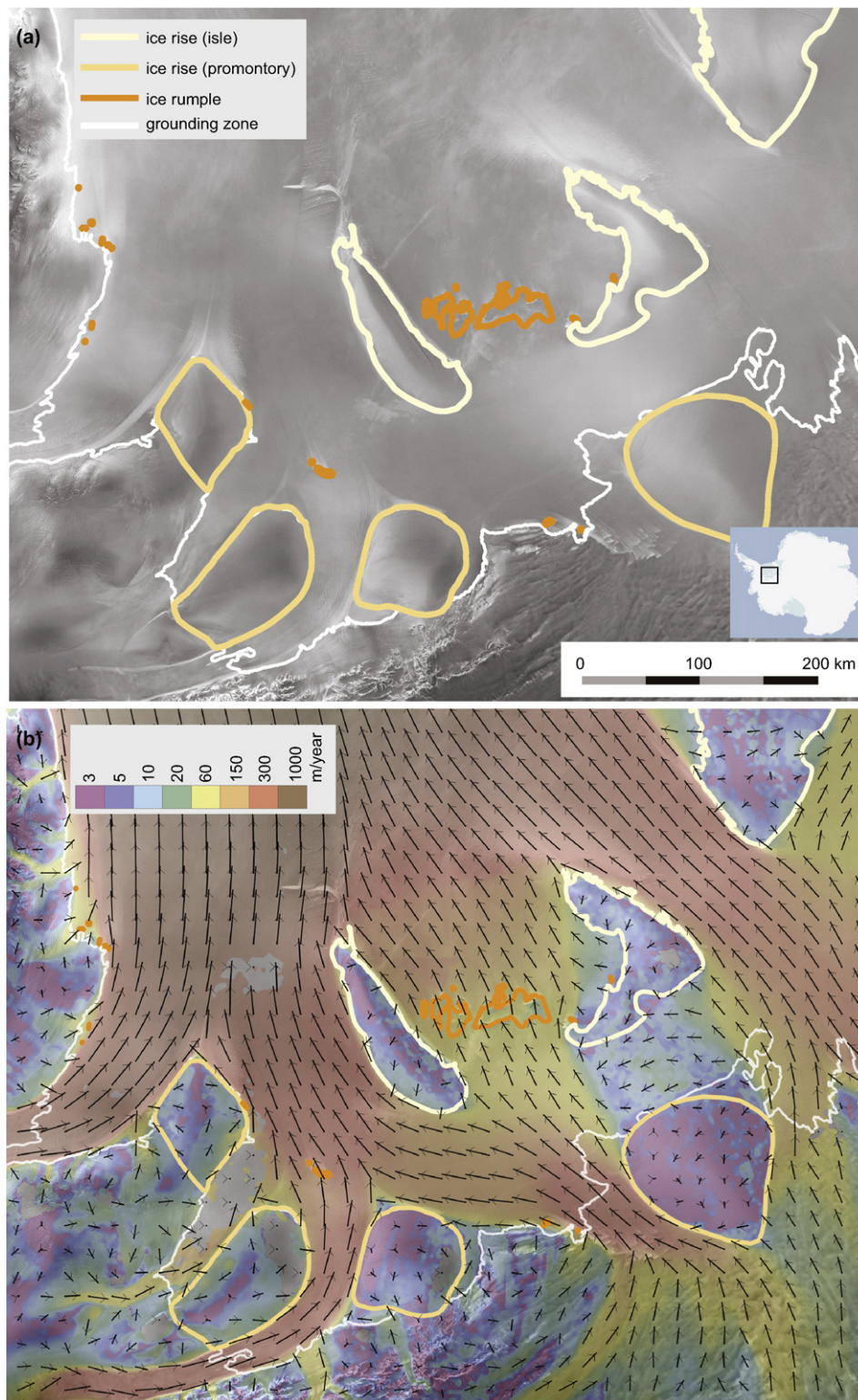
Fig. 1. Ice rises and rumples in the Ronne–Filchner Ice Shelf, West Antarctica. Inset shows the location. Outlined are ice rises and rumples inventoried in this study (see Appendix A). Bed topography in this region and names of these ice rises and rumples are shown in Fig. 6b. The grounding zone of the ice sheet is also shown (Bindschadler et al., 2011). (a) Morphological structures associated with ice rises and rumples visible in Radarsat-2 satellite imagery (Jezek et al., 2002). Brightness changes are associated with surface-slope variations of major ice rises, as well as crevasses and rifts in the ice shelf. (b) Ice flow field (Rignot et al., 2011a) perturbed by ice rises and rumples. Arrow lengths are proportional to the logarithm of ice-flow speeds.
