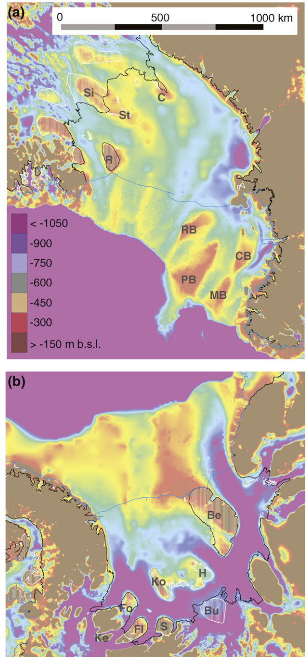
Fig. 6. Elevated bed topography beneath ice rises and rumpled in the Ross (a) and Weddell (b) Sea Embayments. Bed elevations are referenced to the GLO4C geoid (Fretwell et al., 2013); geoid heights are ~40 m in the Ross Sea and ~20 m in the Weddell Sea. Outlined are the grounding zone (black; Bindshadler et al., 2011) and current ice-shelf’s calving front (blue; Scientific Committee on Antarctic Research, 2012). Inventoried ice rises and rumpled (Appendix A) are hatched, and labels are given to major ice rises. In Panel (a), labeled are Siple Dome (Si), Roosevelt Island (R), Crary Ice Rise (C), and Steershead Ice Rise (St), as well as likely locations of ice rises during the LGM (Shipp et al., 1999): Crary Bank (CB), Mawson Bank (MB), Pennell Bank (PB) and Ross Bank (RB). In panel (b), labeled are the current ice rises and rumpled: Berkner Island (Be), Henry Ice Rise (H), Korff Ice Rise (K), Bungenstock Ice Rise (Bu), Skytrain Ice Rise (S), Kealey Ice Rise (Ke), Fletcher Promontory (Fl), and Fowler Peninsula (Fo).
