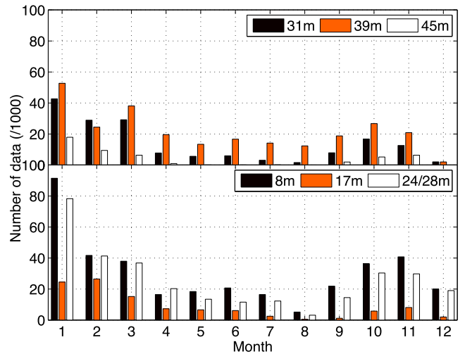
Figure 2. Number of data samples collected by each sonic every month from 2006 November to 2012 May. One data sample corresponds to 1 min of measurement. Top: the three upper sonics. Bottom: the three lower ones (the third was at height 28 m in 2006–2007, then at height 24 m).
