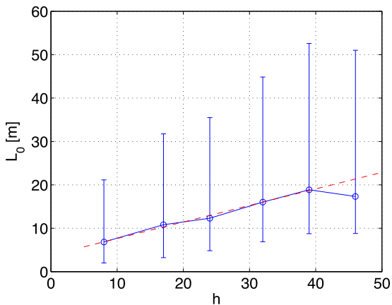
Figure 6. Outer scale L_0 as a function of the height of the anemometer. Error bars are the intervals containing 50 per cent of the data. The dashed line is a least-squares fit obtained on the five first points.
