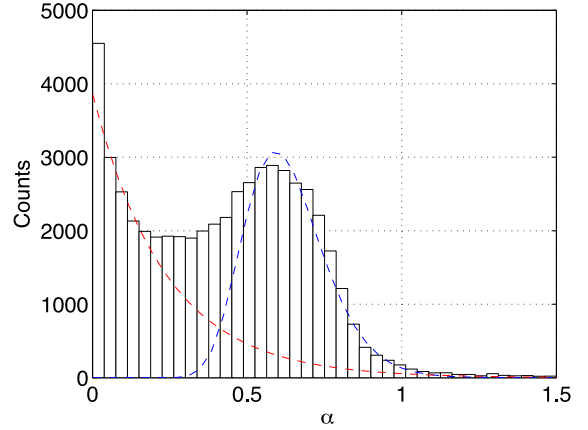
Figure 4. Histogram of the slopes \alpha of the structure functions D_T(\rho) of the sonic temperatures in the interval \rho \in [0.6 \text{ m}, 4 \text{ m}] . This histogram was computed from all six sonics data collected during the years 2008–2011. The dashed lines are (i) a negative exponential fit of the first part of the histogram for small values of \alpha , and (ii) a lognormal fit of the bump centred at \alpha = 0.6 .
