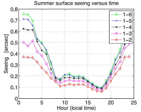
Figure 14. Hourly median values of the SL seeing \epsilon_s in summer (the period considered here is 2008 December where all six sonics were in operation), integrated between 8 m and the altitude of each sonic. Label such as ‘1–3’ means an integration between the first sonic ( h = 8 m) and the third ( h = 24 m).
