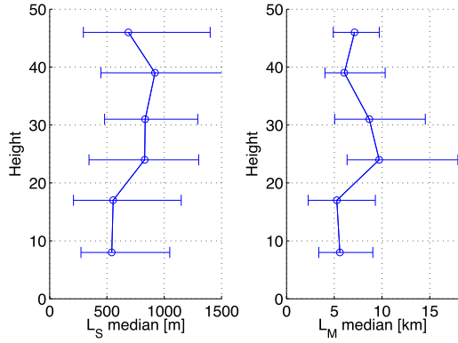
Figure 9. Vertical profiles of L_S and L_M computed from 4-days structure functions for each sonic. Error bars represent the 50 per cent confidence interval.
