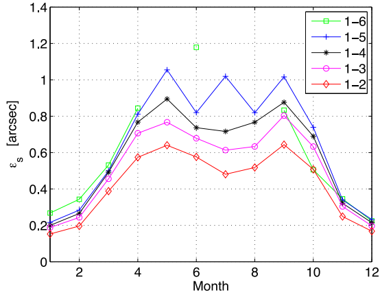
Figure 13. Monthly median values of the SL seeing \epsilon_s integrated between 8 m and the altitude of each sonic. Label such as ‘1–3’ means an integration between the first sonic ( h = 8 m) and the third ( h = 24 m).
