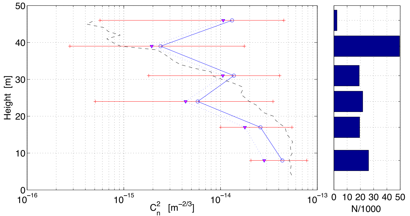
Figure 11. C_n^2 median profile for the period April–October. Blue circles: values corrected from the bias as described in Section 4.5. Triangles: raw values. Error bars are the 50 per cent confidence interval around the blue circles. The dashed line is the median profile obtained in 2005 (March 15 to October 19) from in situ radiosoundings. The histogram on the right is the number N of valid sonic data at each altitude.
