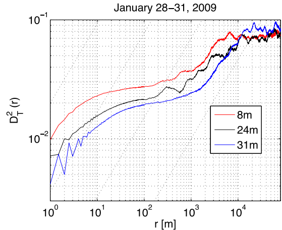
Figure 8. Large-scale structure function calculated on 4 d of data from 2009 Jan. 28 to Jan. 31. Oblique dashed lines have a slope 2/3.
