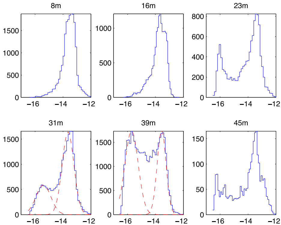
Figure 12. Histograms of \log C_n^2 at different heights for the period April–September. Data corresponding to heights 31 and 39 m were fitted by a sum of two Gaussian (dashed red curves).
