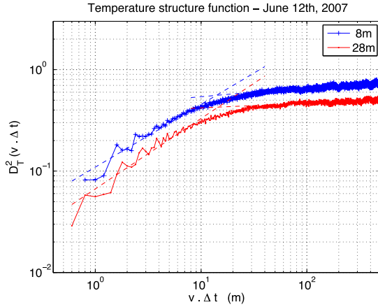
Figure 3. Structure functions computed from data taken on 2007 June 12. The upper curve corresponds to the 8 m sonic, and the lower one to the 28 m sonic. The dashed lines are least-squares fits of the inertial domain and on the saturation domain (large values of \bar{v}\Delta t ).
