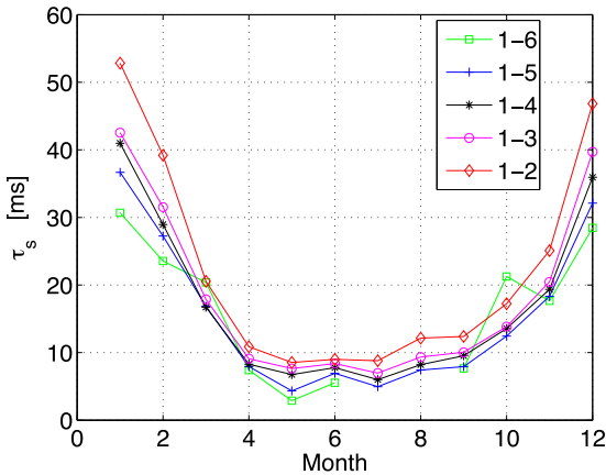
Figure 15. Monthly median values of the coherence time SL \tau_s integrated between 8 m and the altitude of each sonic.
