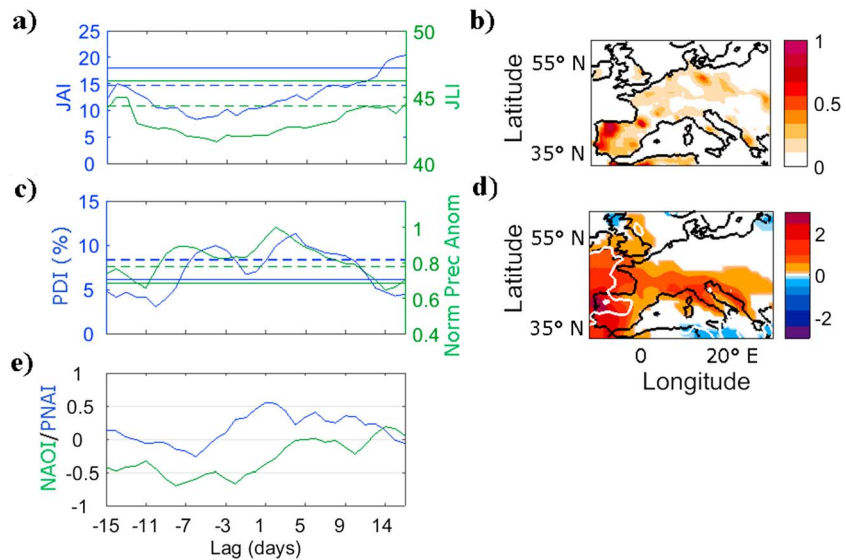
Figure 2. (a) JAI (200–400 hPa, blue) and JLI (200–400 hPa, green). (b) Composite PD values over lags -5 to +5 days, normalized to the interval (0, 1) . (c) PDI (blue) and rainfall anomaly (green) ( \text{mm d}^{-1} ) over lags -5 to +5 days; only anomalies exceeding the 95% confidence level derived from a random Monte Carlo sampling procedure are shown. (d) Mean composite precipitation anomalies over lags -5 to +5 days; only anomalies exceeding the 95% confidence level derived from a random Monte Carlo sampling procedure are shown. (e) PNAI (blue) and NAOI (green) values at multiple time lags. All values and lags refer to the North American cold spells. The continuous horizontal lines in Figures 2a and 2c mark the wintertime average values. The dashed horizontal lines mark the (a) 5th and (b) 95th percentiles, derived from a random Monte Carlo sampling procedure. The rainfall anomalies in Figure 2c are area-weighted values cumulated over all gridboxes in the domain, summed over 3 day periods and normalized to have a maximum value of +1 . The abscissa in Figure 2c indicate the central days of the 3 day intervals. The white contours in Figure 2d mark areas where at least two thirds of the events agree on the sign of the anomalies. The data covers the same range as Figure 1.
