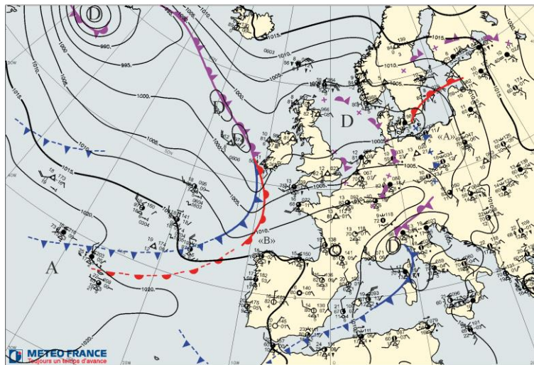
(b) SURFACE ANALYSES 1200 UTC 15 OCT 2012
