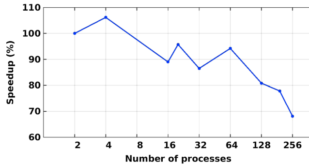
Figure 1. Parallel speedup of the code. The blue curve shows the real performance.)
