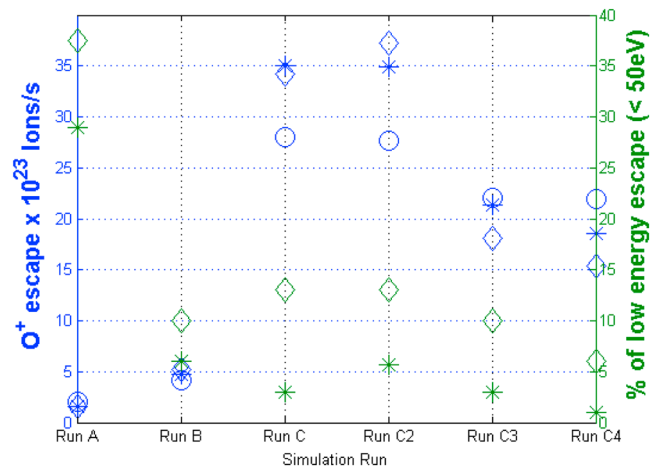
Figure 6. O + ion escape from different integration surfaces (diamond: spherical shell at the altitude of 1200 km; asterisk: shell at 3600 km; circle: the outer simulation domain) and for the different simulation runs (blue symbols). Green symbols represent the contributions of the lower energy population to the total escape.
