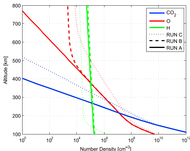
Figure 2. Density profiles for the CO 2 (blue), O (red), and H (green) used in the simulations. Full lines represent the profiles used for RUN A, the dashed lines for RUN B while the dotted lines are for RUN C.
