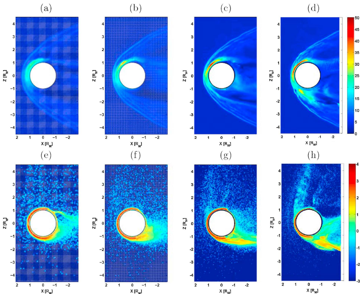
Figure 4. Simulation results of (a, e) RUN C4, (b, f) RUN C3, (c, g) RUN C, and (d, h) RUN C2. The spatial resolution improves from left to right ( \Delta x = 180, 130, 80, \text{ and } 50 km). Figures 4a–4d show the total magnetic field (in nT) in the XZ plane while Figures 4e–4h display the O^+ ion number density (in \text{cm}^{-3} , log scale) in the same plane, plane containing the convection electric field.
