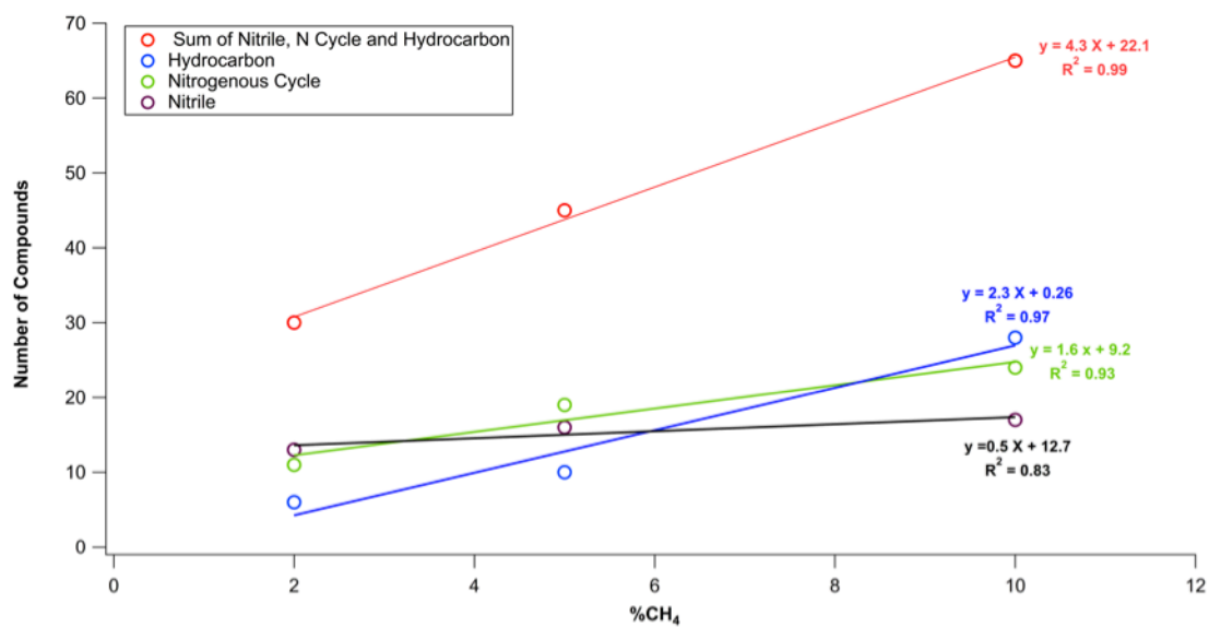
Figure 5 Evolution of the number of compounds released in each chemical family versus %CH 4
