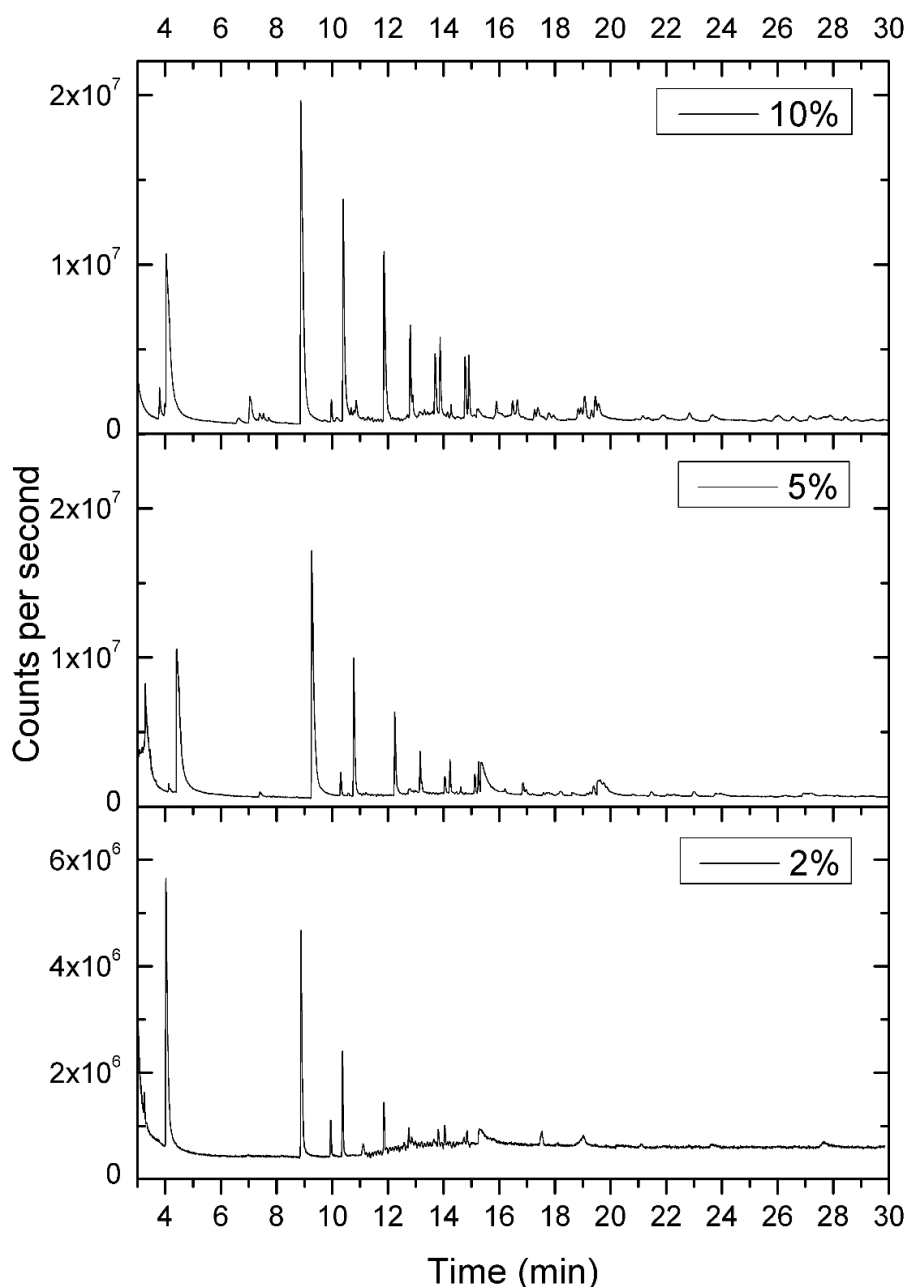
Figure 4 Chromatograms obtained after a 400°C pyrolysis of 2%-tholins (bottom), 5%-tholins (middle) and 10%-tholins (top) with the Q-PLOT column.
