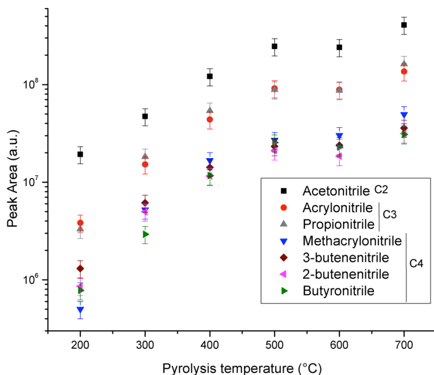
Figure 7 Evolution of the peaks area with pyrolysis temperature for major nitriles identified in 10%-tholins pyrolysates.
