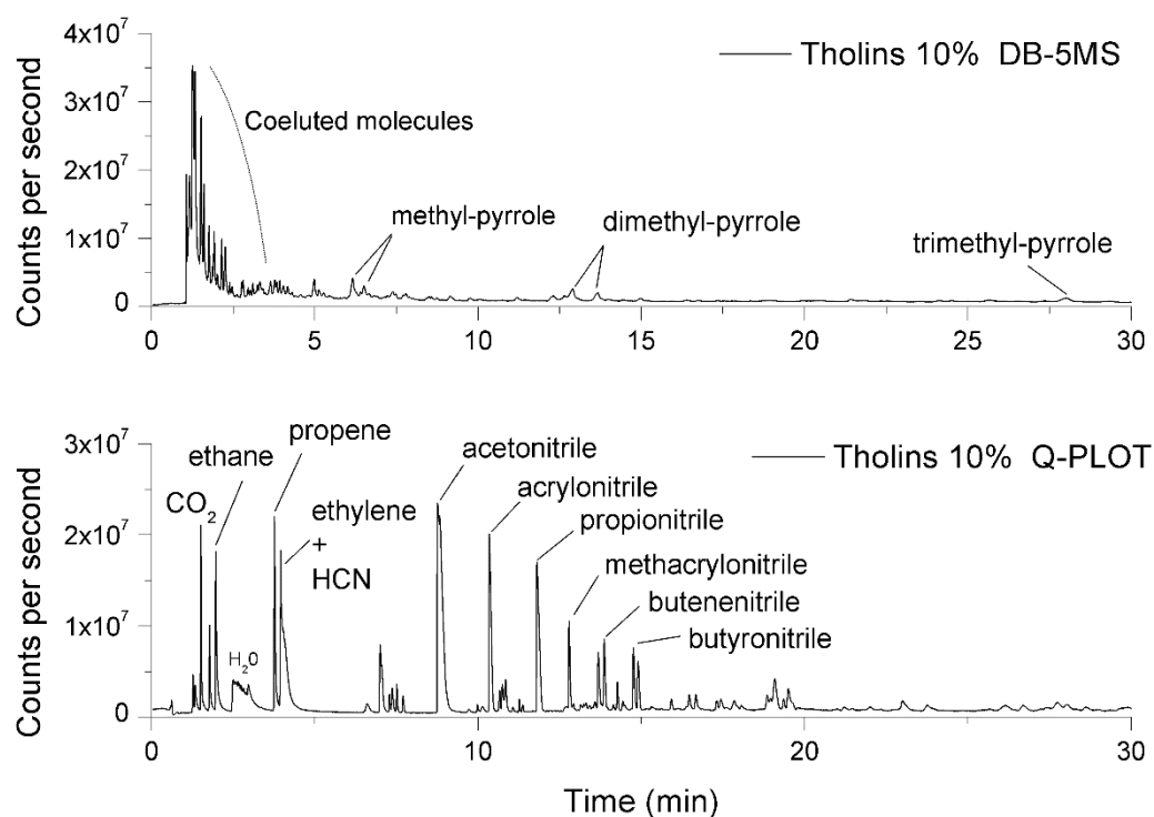
Figure 1 Chromatograms obtained after a 600°C pyrolysis of 10%-tholins, with the DB-5MS column (top) and Q-PLOT column (bottom).
