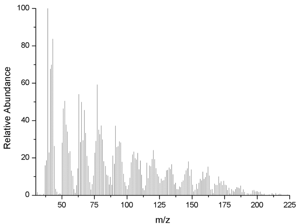
Figure 6: Mass-pattern obtained after a 600°C pyrolysis of the 10%-tholins with the DB-5MS column.
