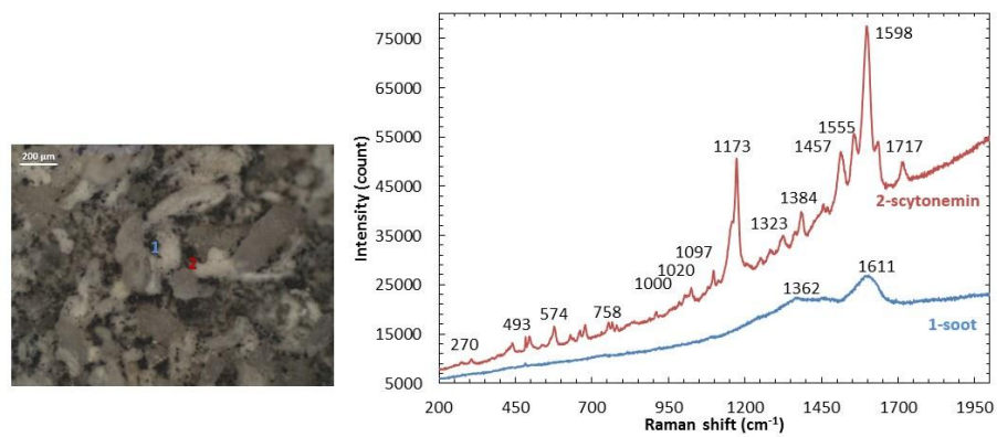
Figure 10: Optical micrograph on the limestone from Saint-Denis and associated Raman spectra ( \lambda=532 nm).
