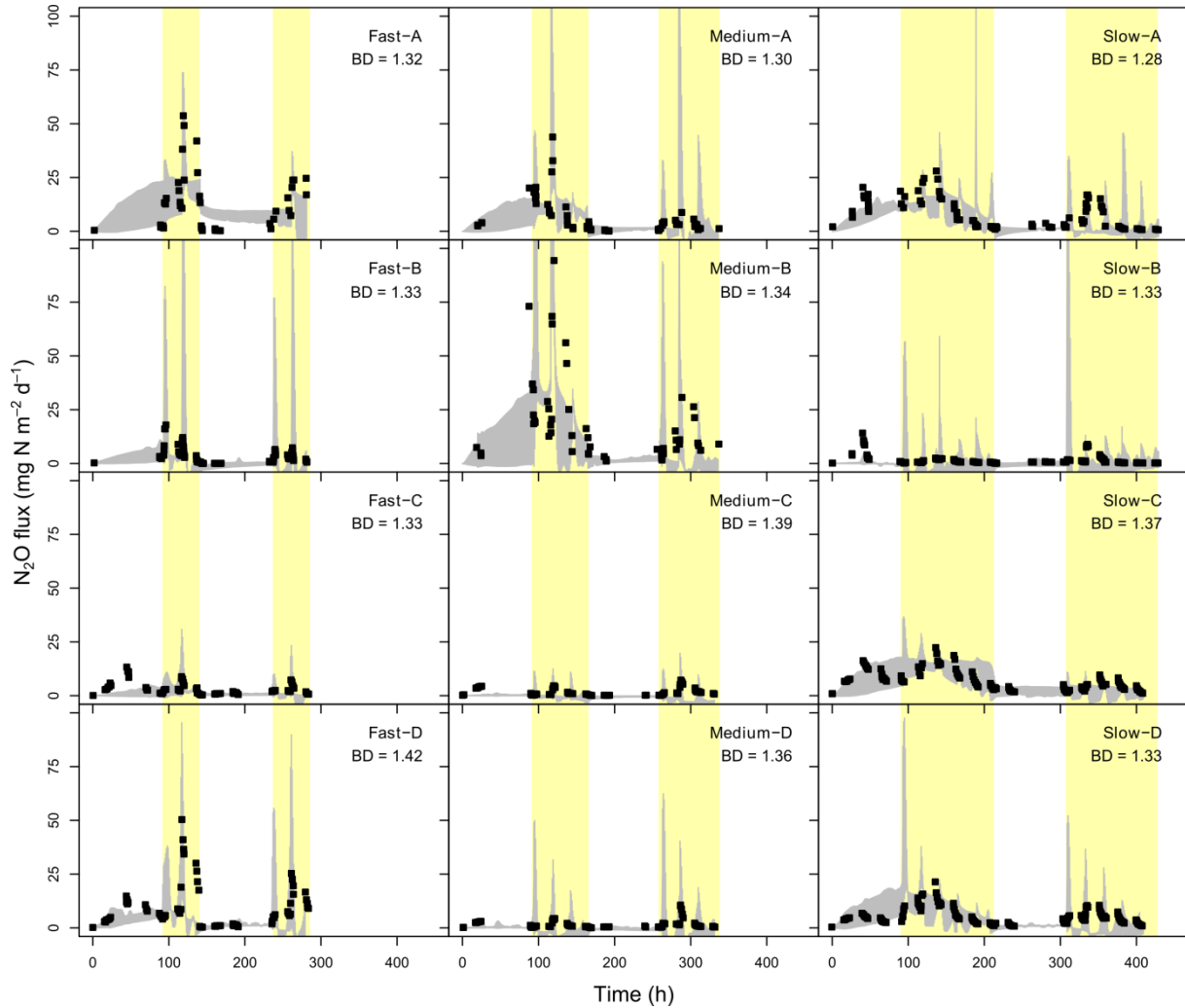
Fig. 5 Measured (black squares) and 95% confidence interval of simulated N 2 O fluxes (grey areas). Sample names refer to the number of decreasing pressure heads applied during one wetting-drying cycle (Fast: 3 values, Medium: 4 values, Slow: 6 values, BD: bulk density in g cm -3 ). Yellow areas represent the drying phases, and white areas the wetting phases
