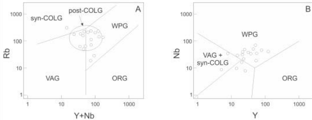
Fig. 10. Rb versus (Y + Nb) and Nb versus Y diagrams (Pearce et al., 1984 and Pearce, 1996).
