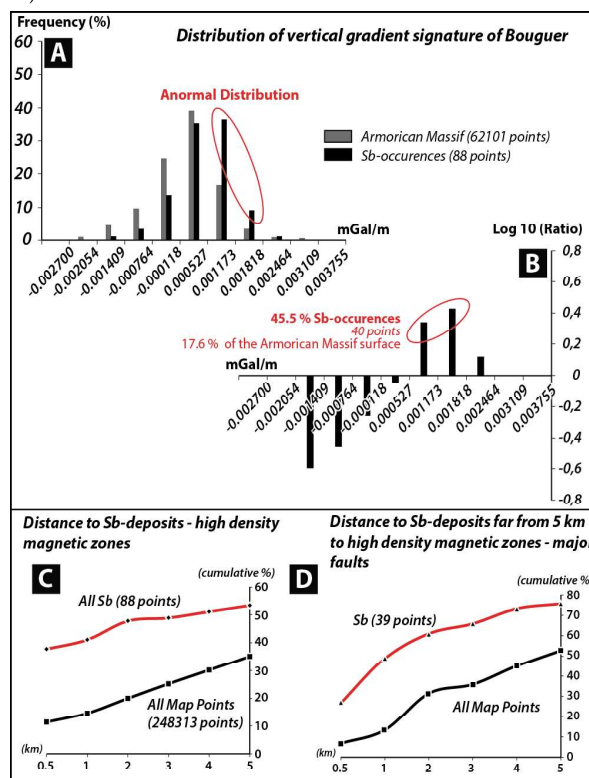
Figure 2. A. Frequency histogram of vertical gradient of Bouguer anomaly signature. B. Frequency log10 (Sb-values/Armorican Massif-values) histograms. C. Spatial proximity analysis calculated among Sb-deposits and all map points and high density magnetic zones. D. Spatial proximity analysis calculated among Sb-deposits located at more 5 km to high-density magnetic zones and to all map points and major faults.
