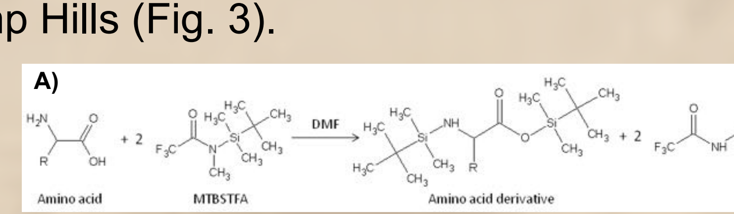
Fig. 5: SAM wet chemistry. A) MTBSTFA derivatization reaction. B) SAM carousel containing 7 MTBSTFA cups (detailed in C))
