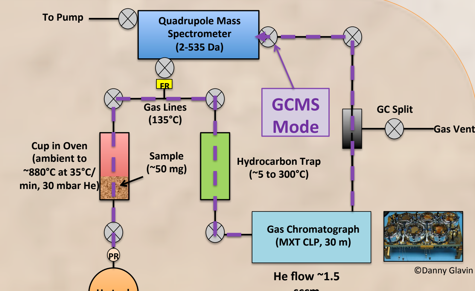
Fig. 4: Simplified gas flow diagram for the GCMS mode of SAM
