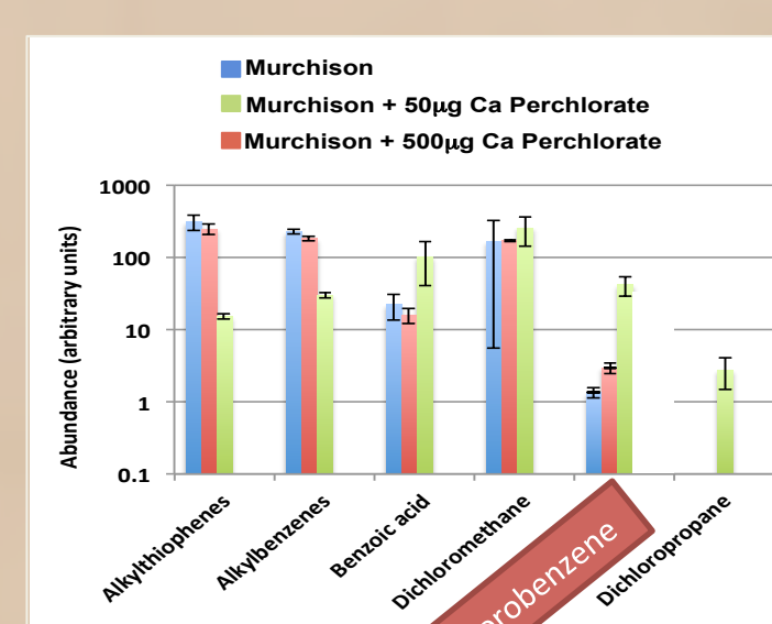
Fig. 8: formation of CBZ from Murchison pyrolysed in presence of perchlorate
