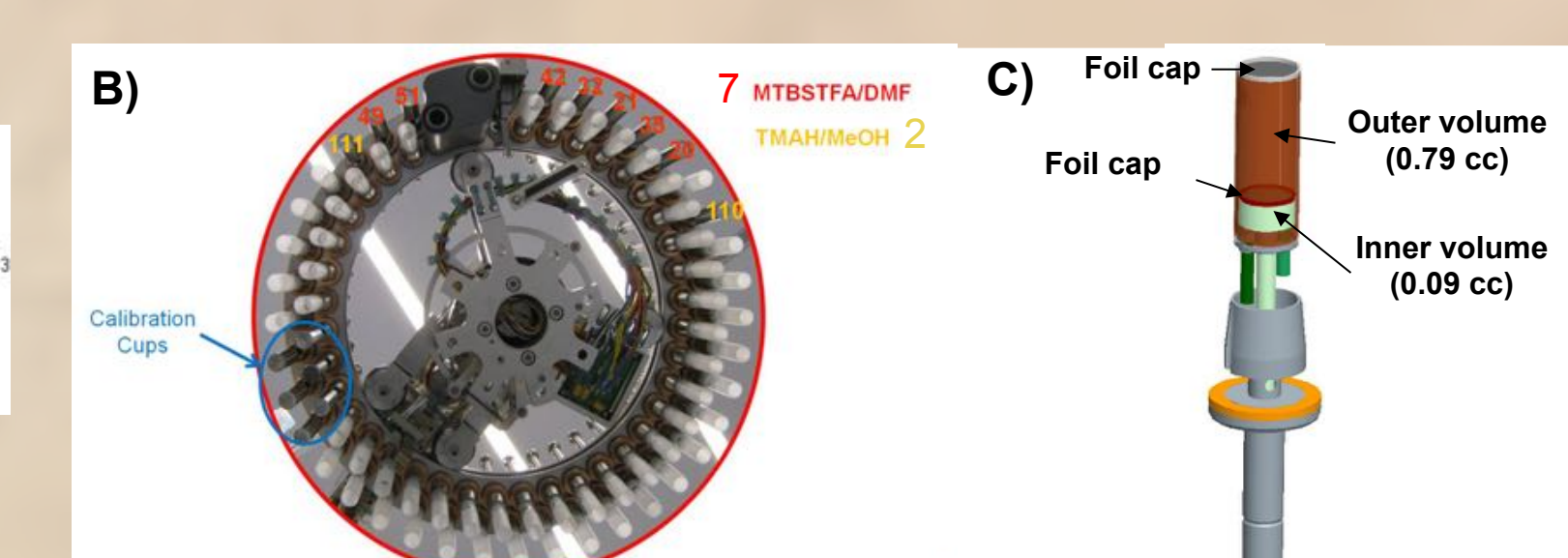
Fig. 5: SAM wet chemistry. A) MTBSTFA derivatization reaction. B) SAM carousel containing 7 MTBSTFA cups (detailed in C))
