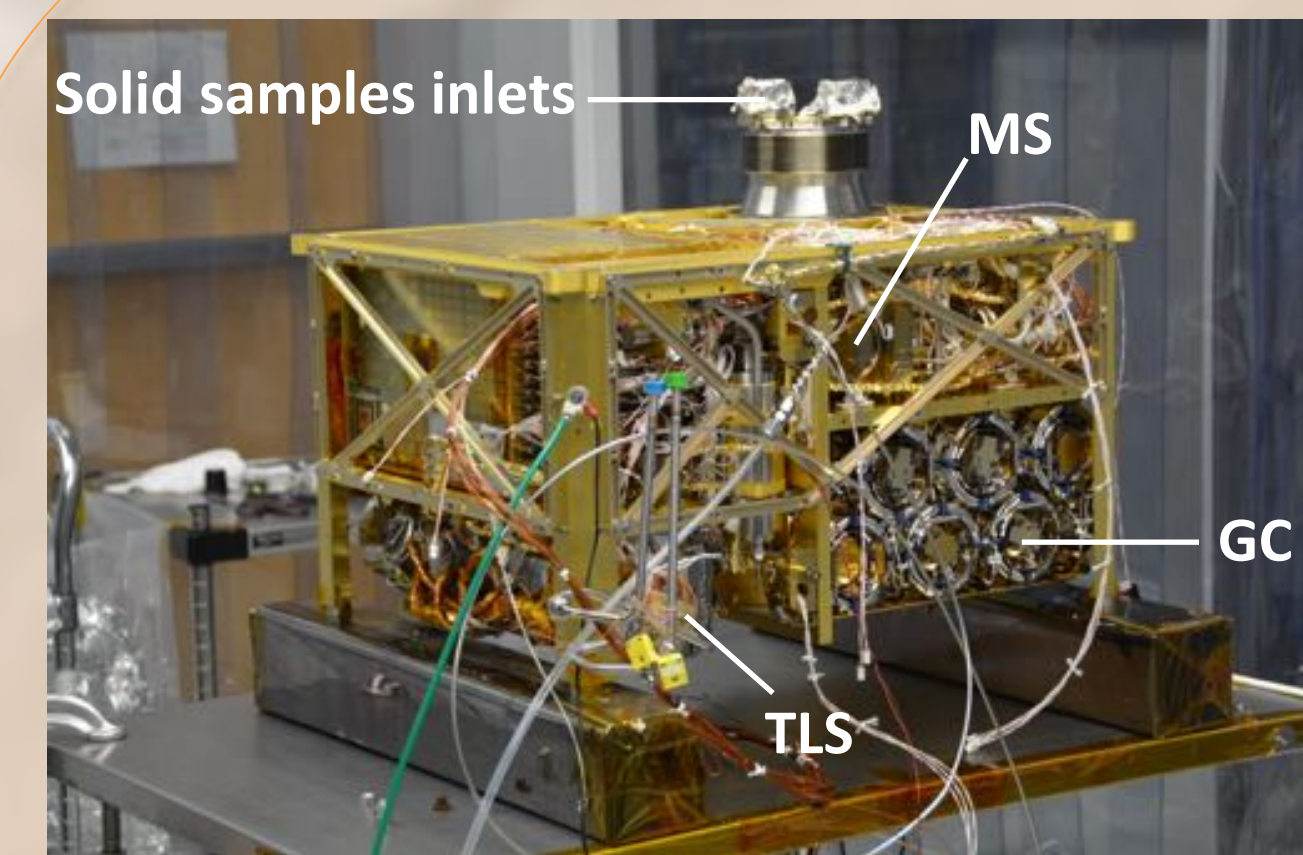
Gas Chromatograph (GC) – Separates individual compounds from a mix Mass Spectrometer (MS) – Identifies molecules from their mass Tunable Laser Spectrometer (TLS) – Molecules and Isotopes
