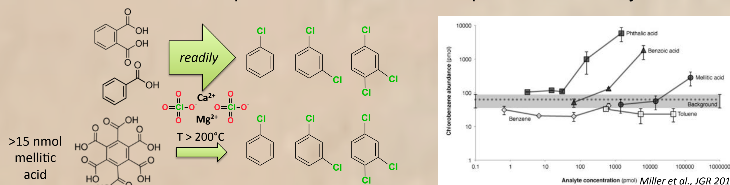
Fig. 7: laboratory experiment show that benzoic, phthalic and mellitic acid, heated in the presence of perchlorate, would form chlorobenzene, dichlorobenzene and trichlorobenzene, and that the abundance of CBZ depends on the initial abundance of the aromatic hydrocarbon.
