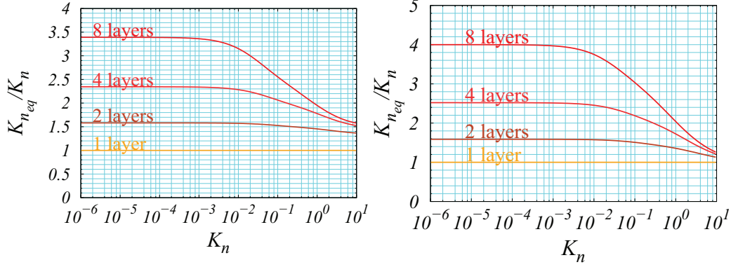
FIG. 3. (Color online) Graph of K_{n_{eq}} for one, two, four, and eight layers: (a) self-similar case and U_{dT} = Q/H , (b) \beta_i = 1 and U_{dT} = Q/H_{eq} .
