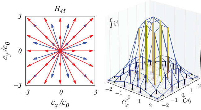
FIG. 5. (Color online) Two-dimensional velocity lattice of \mathcal{H}_{45} (left). f^e distribution of \mathcal{H}_{34} (right).
