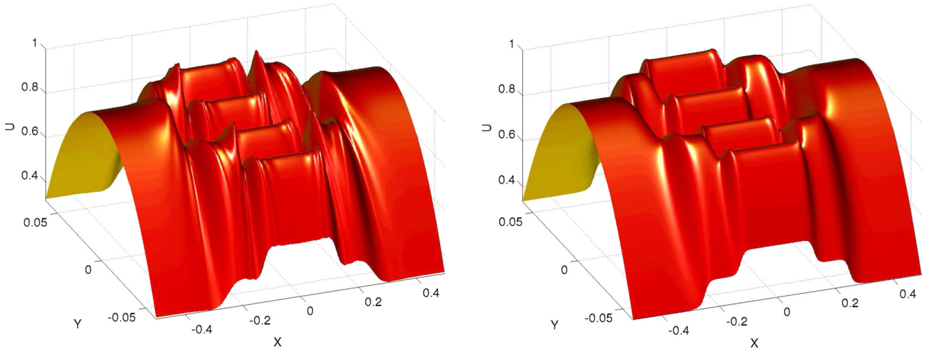
FIG. 6. (Color online) Velocity profiles for K_n = 0.16 : (a) BGK, (b) CFD.
