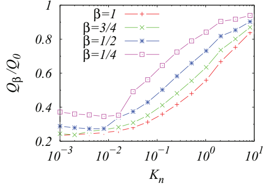
FIG. 10. (Color online) Q_\beta/Q_0 ratio versus K_n for \beta = 1/4, 1/2, 3/4 , and 1, where Q_\beta is the flow rate of the network for which the internal wall length is \beta L .
