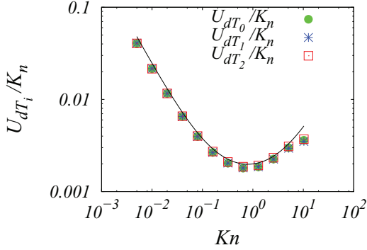
FIG. 8. (Color online) BGK simulation: total flow velocity for sections 0, 1, and 2 of Fig. 1, reduced to Knudsen number. The continuous curve is the theoretical prediction.
