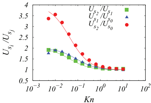
FIG. 9. (Color online) BGK simulation: ratio of slip-velocities for sections 0, 1, and 2 of Fig. 1. The continuous curve is the theoretical prediction given by Eq. (28).
