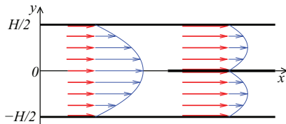
FIG. 2. (Color online) (a) Schematics of U_{dP} and U_s profiles. (b) Stream lines in the elementary network, \beta = 1/2 . The Knudsen number in sections labeled 1 is twice K_n in sections labeled 0.
