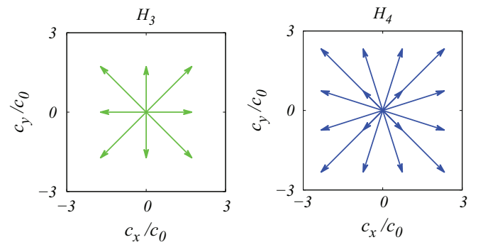
FIG. 4. (Color online) Two-dimensional velocity lattice based on \mathcal{H}_3 (a) and \mathcal{H}_4 (b).
