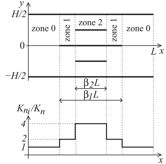
FIG. 1. Schematics of the elementary network with its internal walls.
