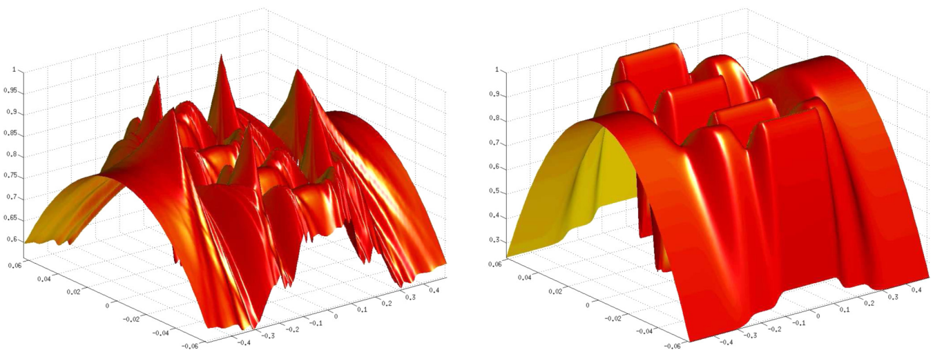
FIG. 7. (Color online) Velocity profiles for K_n = 0.64 : (a) BGK, (b) CFD.
