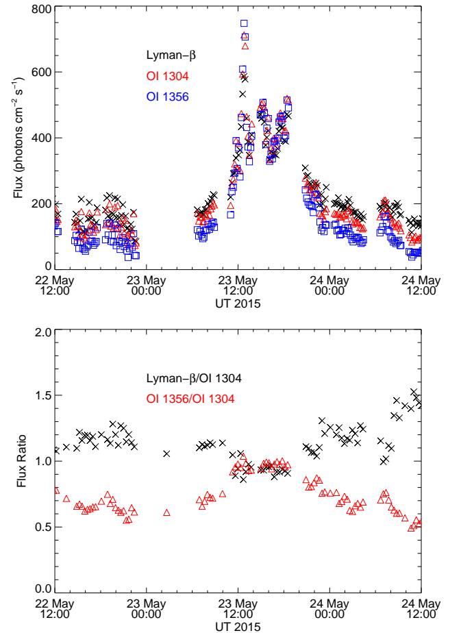
Figure 1. Temporal variation of the atomic hydrogen and oxygen emissions above the limb on 2015 May 22–24 (top). Individual error bars are not shown but the 1- \sigma statistical uncertainty for all points is <5\% . The bottom panel shows the variation in relative intensities of these emissions.
