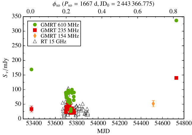
Figure 3. Flux density values of LS I +61 303 as a function of the MJD obtained from all the analysed GMRT data (2005–2008). We show the superorbital phase, \phi_{so} , on the top x -axis. The green circles represent the 610-MHz data, the red squares the 235-MHz data, and the orange diamond the 154-MHz ones. The grey triangles represent the daily averages of the RT data at 15 GHz. Error bars represent 1\sigma uncertainties (smaller than the data points when they are not visible). We note that the source exhibits larger flux densities during the isolated GMRT observations (at superorbital phases of \phi_{so} \approx 0.80 – 0.95 ) than during the GMRT monitoring ( \phi_{so} \approx 0.2 ).
