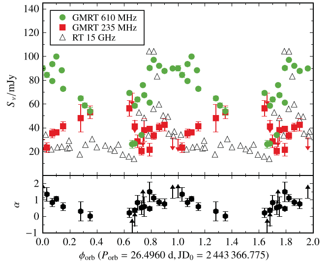
Figure 5. Top: folded light curve with the orbital period of the data shown in Fig. 4. The 610 MHz data show a quasi-sinusoidal modulation with enhanced emission at \phi_{orb} \approx 0.8 – 1.1 , whereas the 15-GHz outbursts take place at \phi_{orb} \approx 0.8 with a fast decay. The 235 MHz light curve is almost anticorrelated with the one observed at 610 MHz. Bottom: spectral index \alpha derived from the GMRT data presented above. Open hexagons represent the spectral index from the isolated GMRT data (not shown on top). Error bars represent 1\sigma uncertainties and the arrows represent the 3\sigma upper/lower limits.
