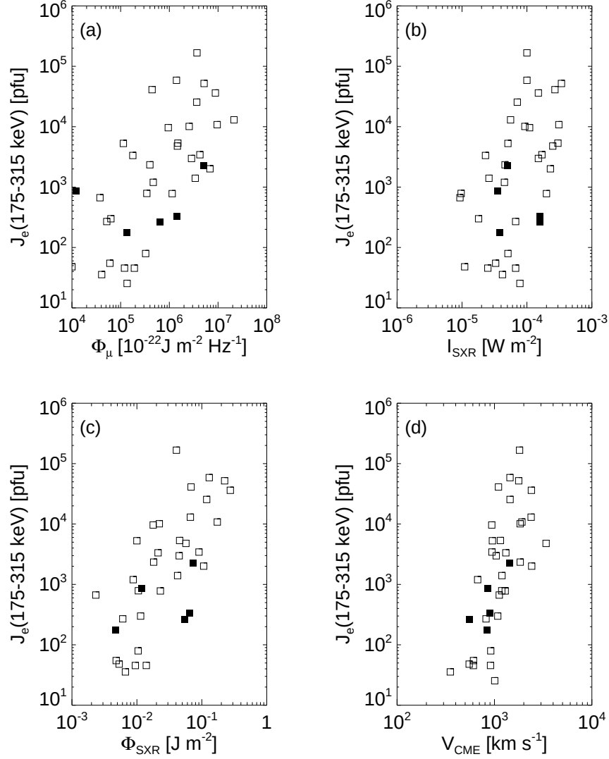
Figure 4. Scatter (log-log) plots of the electron peak intensity J_e(175 \text{ keV}) versus microwave peak fluence \Phi_\mu , peak SXR flux I_{\text{SXR}} , start-to-peak SXR fluence \Phi_{\text{SXR}} and CME speed V_{\text{CME}} . Unconfined events are plotted by open squares, confined events by filled squares.
