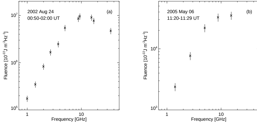
Figure 1. The microwave fluence spectra of two events with different values of the quality flag. (a) An event with quality flag 1, indicating that the maximum of the fluence spectrum lay within the observed frequency range (combined data from NoRP and one RSTN station). (b) An event with a quality flag 2, where the maximum of the fluence spectrum occurred outside of, but close to the observed frequency range (data from the San Vito RSTN station).
