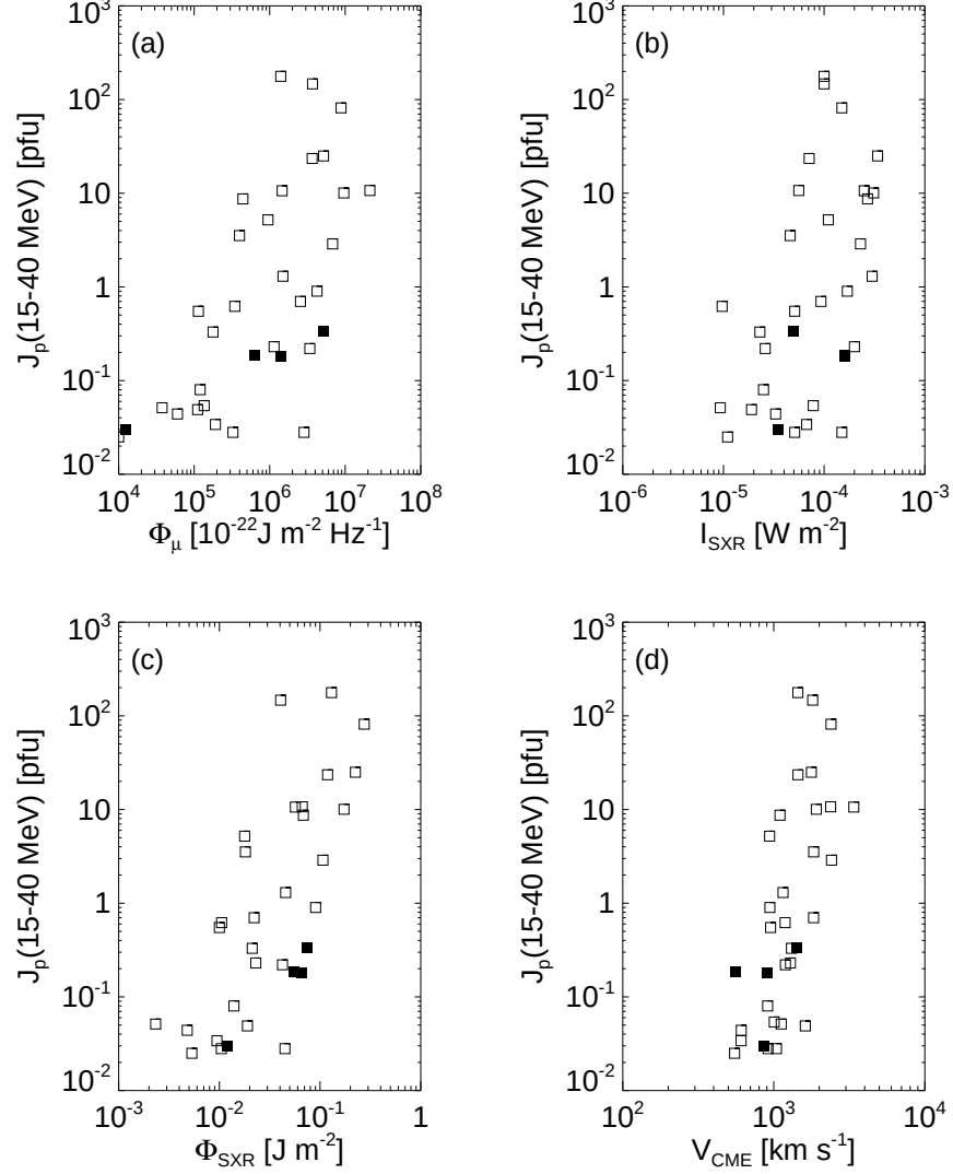
Figure 3. Scatter (log-log) plots of proton peak intensity J_p versus microwave peak fluence \Phi_\mu , peak SXR flux I_{\text{SXR}} , start-to-peak SXR fluence \Phi_{\text{SXR}} and CME speed V_{\text{CME}} . Unconfined events are plotted by open squares, confined events by filled squares.
