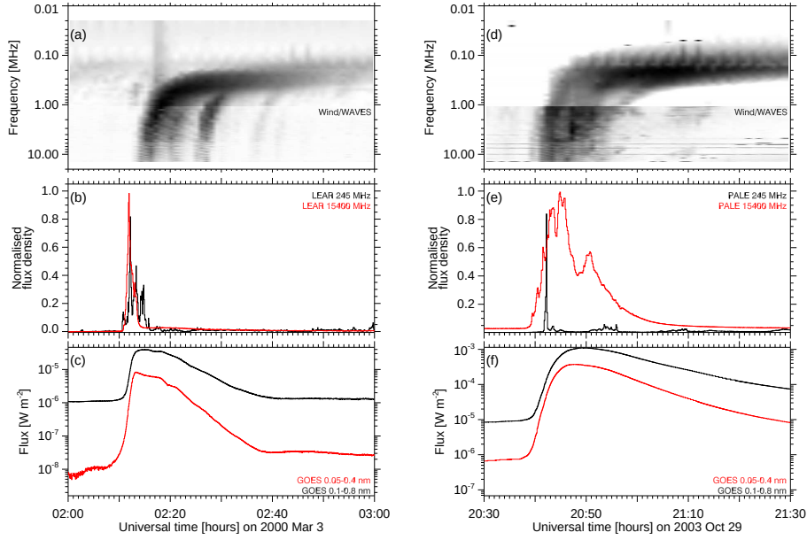
Figure 2. Time histories of X-ray and radio emissions of a confined and an unconfined event, respectively. (a-c) 3 March 2000, (d-f) 29 October 2003. From top to bottom: (a, d) decametre-to-hectometre (DH)wave emission ( Wind /WAVES); (b, e) flux density time profiles at two frequencies in the microwave (15.4 GHz) and metre wave (245 MHz) range (RSTN Network); and (c, f) soft X-ray flux (GOES; black line 0.1 - 0.8 nm, lightly shaded line - red in the online version - 0.05 - 0.4 nm).
