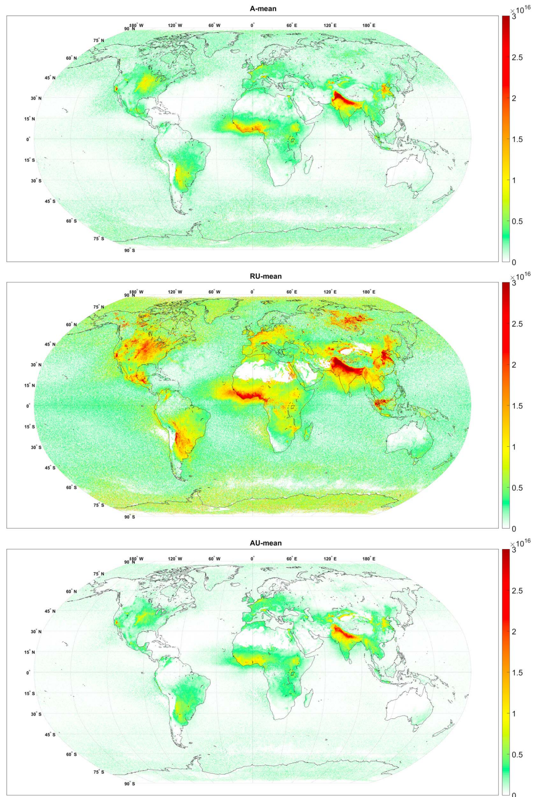
Figure 9. \text{NH}_3 total columns ( \text{molecules}\cdot\text{cm}^{-2} ) distributions from IASI measurements for the year 2013, in a 0.25^\circ by 0.25^\circ grid for the morning overpasses. \text{NH}_3 distributions are a mean of all measurements within a cell following (top) an arithmetic mean (A-mean), (middle) a weighted mean by the relative uncertainty (RU-mean), and (bottom) a weighted mean by the absolute uncertainty (AU-mean).
