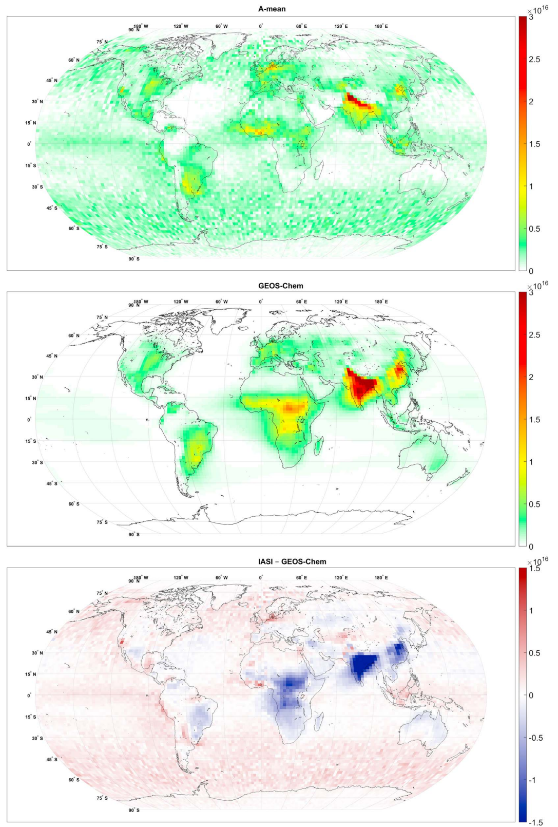
Figure 10. (top) \text{NH}_3 total columns (molecules. \text{cm}^{-2} ) distributions from IASI measurements for the year 2009, in a 2.5^\circ by 2^\circ grid for the morning overpasses. \sigma values were selected by fitting the corresponding GEOS-Chem \text{NH}_3 vertical profiles. (middle) \text{NH}_3 total columns (molecules. \text{cm}^{-2} ) distributions from the GEOS-Chem CTM. (bottom) Differences between \text{NH}_3 total columns (molecules. \text{cm}^{-2} ) distributions measured by IASI and simulated by GEOS-Chem.
