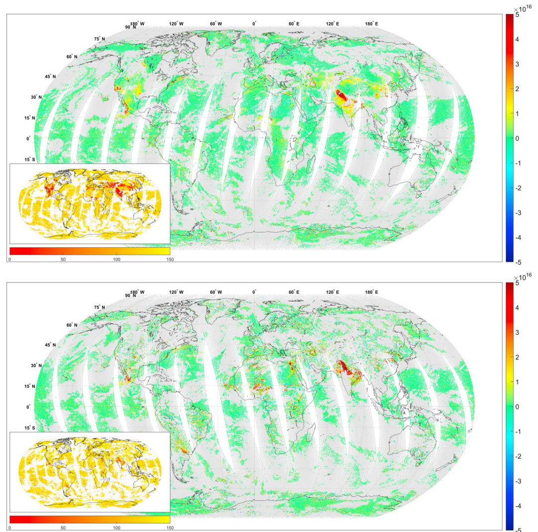
Figure 4. NH 3 total column distributions (molecules.cm -2 ) for (top) the morning and (bottom) the evening overpasses of IASI on Metop-A for 2 June 2013. Associated uncertainty distributions (%) are shown as well (bottom left inset).
