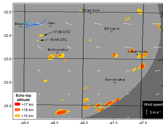
Figure 5. Composite radar image of all convective cells reaching above 15 km detected on 13 March by IPMet radar in the upwind quadrant of Bauru. Black arrows tag the overshooting cells potentially responsible for the hydrated layers shown in Fig. 4 with indication of the UTC of their detection by radar. White arrows represent the mean wind field between 100 and 70 hPa from ERA-Interim reanalysis (18:00 UTC). Blue lines indicate the balloon trajectories (FLASH-B dark blue, Pico-SDLA light blue).
