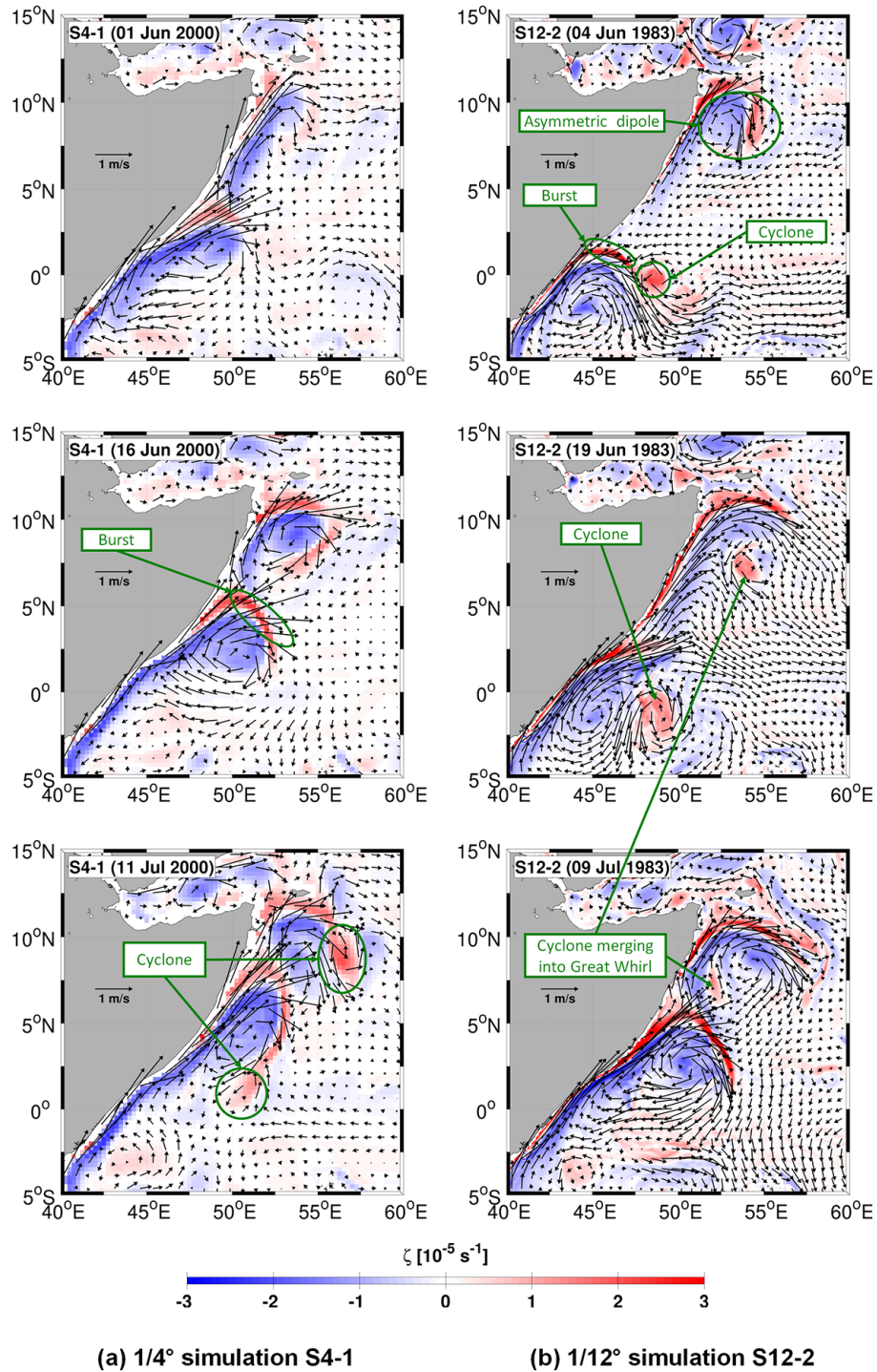
Figure 3. Sequence of relative vorticity ( \zeta ; colour shading; \text{s}^{-1} ) and currents (vectors; \text{m s}^{-1} ) at 50 m, (a) in the 1/4^\circ S4-1 simulation, and (b) in the 1/12^\circ S12-2 simulation. The sequences show the occurrence of the vorticity bursts and their subsequent development into asymmetric dipoles. The two large pools of negative (blue) vorticity are the SG and the GW. The bursts are the filaments of positive (red) vorticity, and the cyclones are the circular features of positive (red) vorticity.
