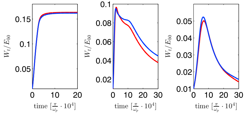
Figure 5. Evolution for the total energy density of waves, W_t , for different levels of density fluctuations and different parameters for the driven beams. Blue lines correspond to density fluctuations with a normal distribution while red lines correspond to fluctuations that obey the Pearson type II distribution. (left) \langle \delta n^2 \rangle^{1/2}/N_0 = 0.005 , v_b = 6v_t , \Delta v_b = 1v_t . (middle) \langle \delta n^2 \rangle^{1/2}/N_0 = 0.02 , v_b = 10v_t , \Delta v_b = 1v_t . (right) \langle \delta n^2 \rangle^{1/2}/N_0 = 0.03 , v_b = 16v_t , \Delta v_b = 1v_t . Figure 5 provide the wave energy density with respect to the corresponding initial energy density of the beam, E_{b0} .
