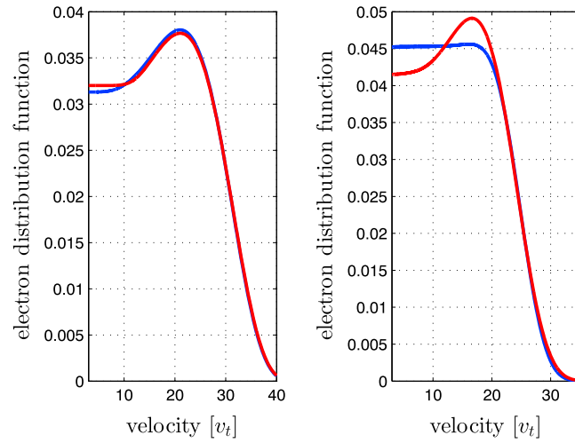
Figure 10. (left) The results of a simulation with a beam with v_b = 20v_t and \Delta v_b = v_t . The level of the density fluctuation, 0.04. The blue line indicates the form of the electron distribution function at time t_1 = 10^6 \pi / \omega_p and the red line at t_2 = 50 \cdot 10^8 \pi / \omega_p . (right) Examples of the electron velocity distribution functions at the end of the first stage of the relaxation process. For both f(v) maximum of the \langle \gamma \rangle is approximately 25 \cdot 10^{-9} \omega / \pi . Initially, the beams have a v_b = 16v_t and a \Delta v_b = 1v_t . The blue line corresponds to a simulation with a level of density fluctuations of 0.01; the red line corresponds to a simulation with a \langle \delta n^2 \rangle^{1/2} / N_0 = 0.04 .
