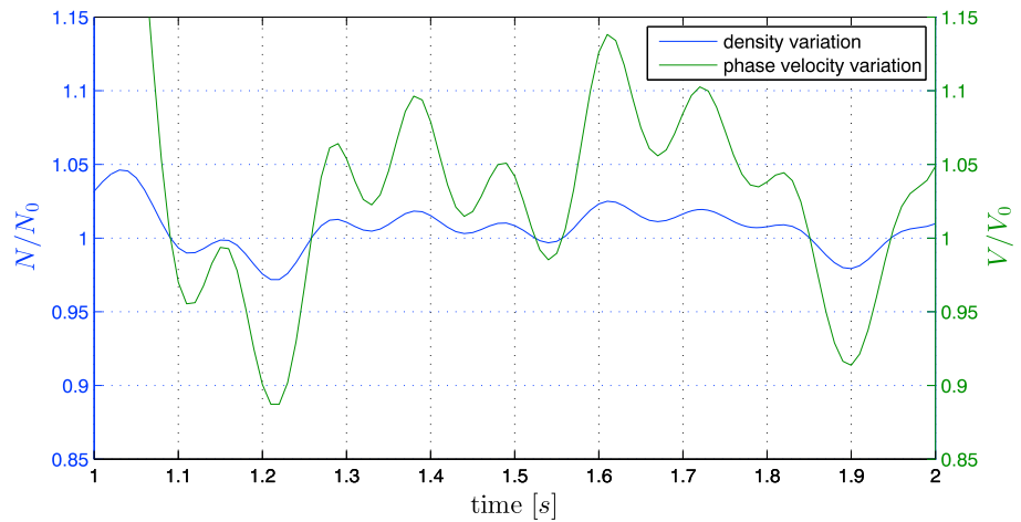
Figure 1. A synthetic time series of density fluctuations reconstructed from the spectrum [Celnikier et al. , 1987] (the blue curve) and corresponding variation of the wave phase velocity (the green curve).
