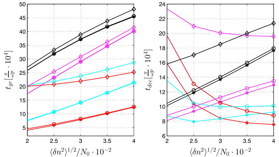
Figure 7. A characteristic time for growth, t_{\text{gr}} , and a characteristic time for decay, t_{\text{dec}} , for the total energy density of waves as a function of the level of the density fluctuation. Different colors that correspond to different beam velocities are as follows: v_b = 10v_t , red; v_b = 12v_t , cyan; v_b = 16v_t , magenta; and v_b = 20v_t , black. Different marks correspond to various initial thermal dispersions of the beam (the same as for Figure 6).
