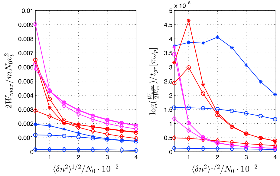
Figure 6. (left) The maximum for wave total energy density, W_{\max} , reached during the relaxation process and (right) the effective growth rate of waves as a function of the level of density fluctuations. W_{\max} is provided with respect to the energy density of the background plasma. W_{\text{in}} and t_{\text{gr}} in Figure 6 (right) represent the initial total energy density of waves and the period of time, over which the wave energy density has grown from W_{\text{in}} to W_{\max} , respectively. Results are provided for various parameters of the beam. Colors that correspond to the various velocities of the beam are as follows: v_b = 6v_t , blue; v_b = 10v_t , red; and v_b = 16v_t , magenta. Different marks that correspond to various thermal dispersions of the beam are as follows: \Delta v_b = 0.5v_t , asterisk; \Delta v_b = 1v_t , circle; and \Delta v_b = 3v_t , diamond.
