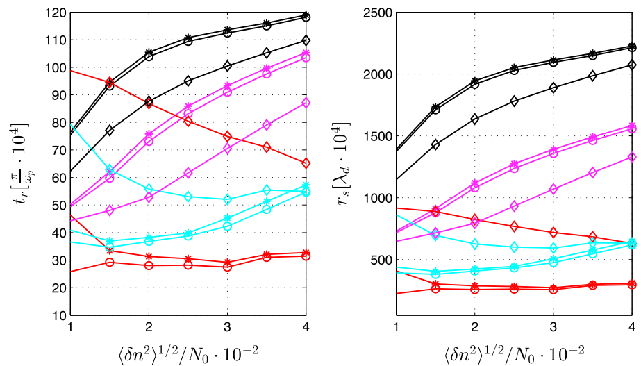
Figure 11. A characteristic time for the relaxation, t_r , and a characteristic spatial scale for the relaxation, r_s , as a function of the level of the density fluctuation. Colors and marks correspond to the various initial beam velocities and the thermal dispersions of the beam (the same as in Figure 7).
