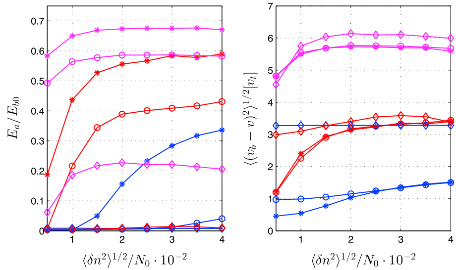
Figure 9. (left) The energy, E_a , for accelerated particles and the thermal dispersion of the beam at the end of relaxation, and (right) \langle (v_b - v)^2 \rangle , as a function of the density fluctuation level. E_{b0} is the initial energy of the beam electrons. Colors and marks correspond to the various initial beam velocities and the thermal dispersions of the beam (the same as in Figure 6).
