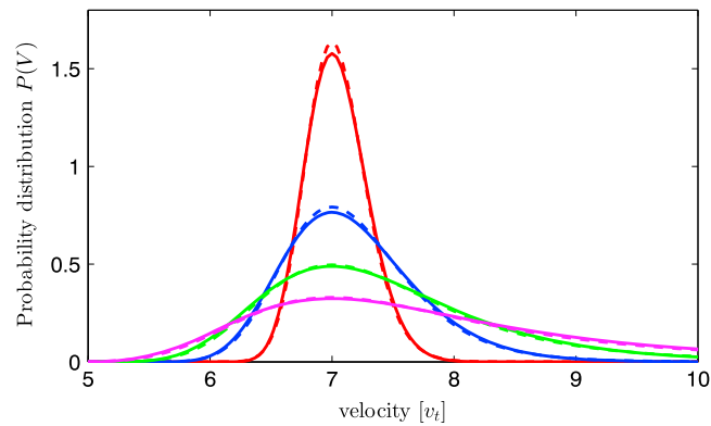
Figure 3. Examples of the probability distribution functions, P_{\omega}(V) , for various fluctuation levels. P_{\omega}(V)dV is the probability that a wave with a ratio of \omega/k_0 = 7v_t will have a phase velocity V at a given interval. P_{\omega} was normalized to one using: \int_0^{\infty} P_{\omega}(V)dV = 1 . Colors that correspond to the various fluctuation levels are as follows: \langle \delta n^2 \rangle^{1/2}/N_0 = 0.005 , red; \langle \delta n^2 \rangle^{1/2}/N_0 = 0.01 , blue; \langle \delta n^2 \rangle^{1/2}/N_0 = 0.015 , green; and \langle \delta n^2 \rangle^{1/2}/N_0 = 0.02 , magenta. Solid lines correspond to density fluctuations obtained using the Pearson type II distribution and the dashed line to density fluctuations obtained using the normal distribution.
