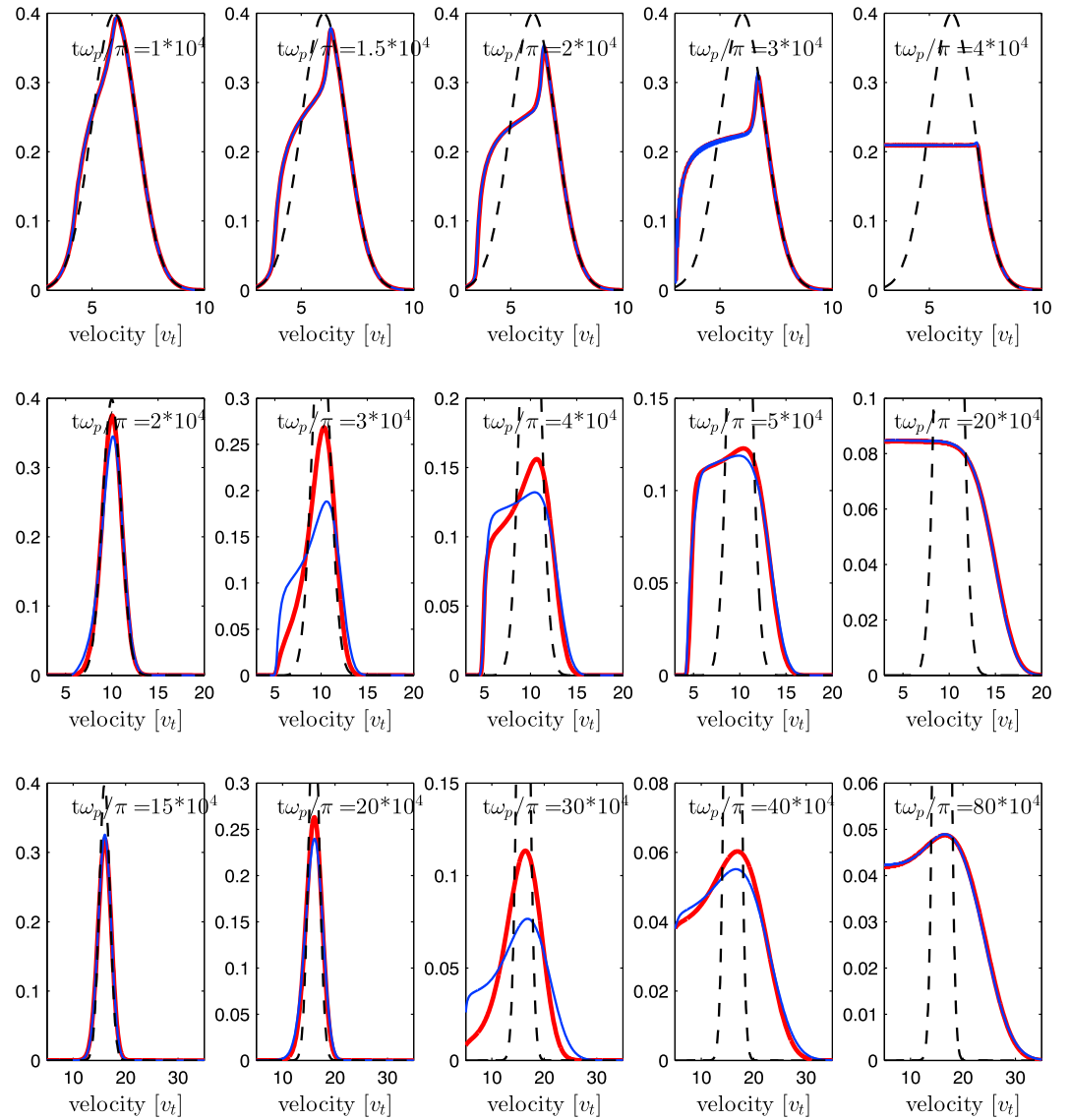
Figure 8. An evolution for electron velocity distribution functions. The core distribution that corresponds to cold electrons of the background plasma was not considered. The dimensionless electron distribution function was normalized to one. Each plot provides a snapshot of the electron distribution function at different moments of time. Colors that correspond to simulations with various distributions for the density fluctuations are as follows: blue, the normal distribution, and red, the Pearson type II distribution. Results were obtained for various parameters of the beam and levels of the density fluctuation. (top row) \langle \delta n^2 \rangle^{1/2} / N_0 = 0.005 ; v_b = 6v_t ; and \Delta v_b = v_t . (middle row) \langle \delta n^2 \rangle^{1/2} / N_0 = 0.02 ; v_b = 10v_t ; and \Delta v_b = v_t . (bottom row) \langle \delta n^2 \rangle^{1/2} / N_0 = 0.03 ; v_b = 16v_t ; and \Delta v_b = v_t .
