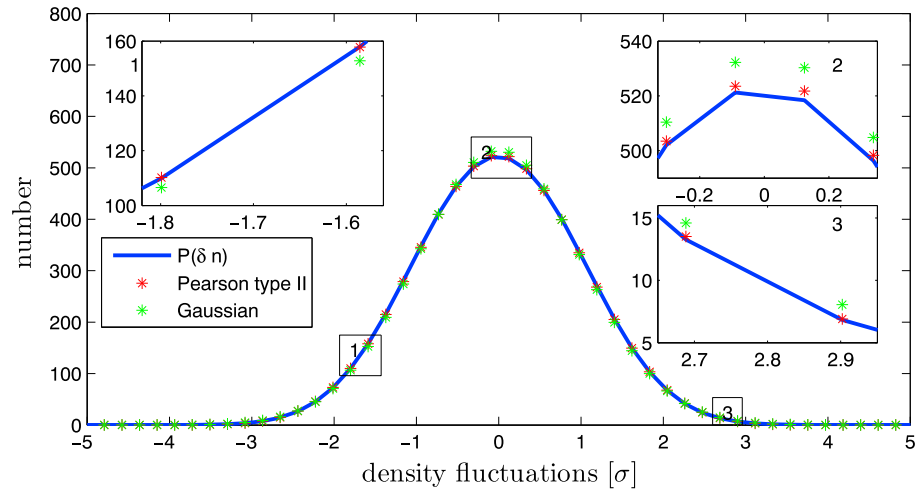
Figure 2. A distribution function for the amplitudes of the density fluctuations. The blue line corresponds to the averaged distribution function obtained from the synthetic time series of the density variation. All of the time series were normalized to its standard deviation, \sigma . Red and green asterisks correspond to the distribution functions obtained from the Pearson type II and the normal probability distribution functions, respectively. Parameters of the fitting probability distribution functions were calculated from synthetic data.
