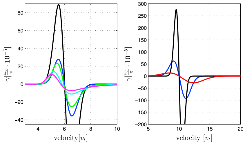
Figure 4. (left) Examples of the growth rate of waves for the various fluctuation levels. Different colors that correspond to the different levels are as follows : \langle \delta n^2 \rangle^{1/2}/N_0 = 0.005 , blue; \langle \delta n^2 \rangle^{1/2}/N_0 = 0.01 , green; \langle \delta n^2 \rangle^{1/2}/N_0 = 0.02 , cyan; and \langle \delta n^2 \rangle^{1/2}/N_0 = 0.04 , magenta. Black line corresponds to the growth rate obtained in the QL approximation for a case of a homogeneous plasma. The driven beam has a Gaussian velocity distribution with v_b = 6v_t and \Delta v_b = 0.5v_t . (right) The growth rate of waves in the QL approximation obtained for the different thermal velocities of the beam. The black line corresponds to \Delta v_b = 0.5v_t , the blue line corresponds to \Delta v_b = 1v_t , and the red line corresponds to \Delta v_b = 2v_t . For all cases v_b = 10v_t . All results are provided for a ratio of n_b/N_0 = 10^{-5} .
