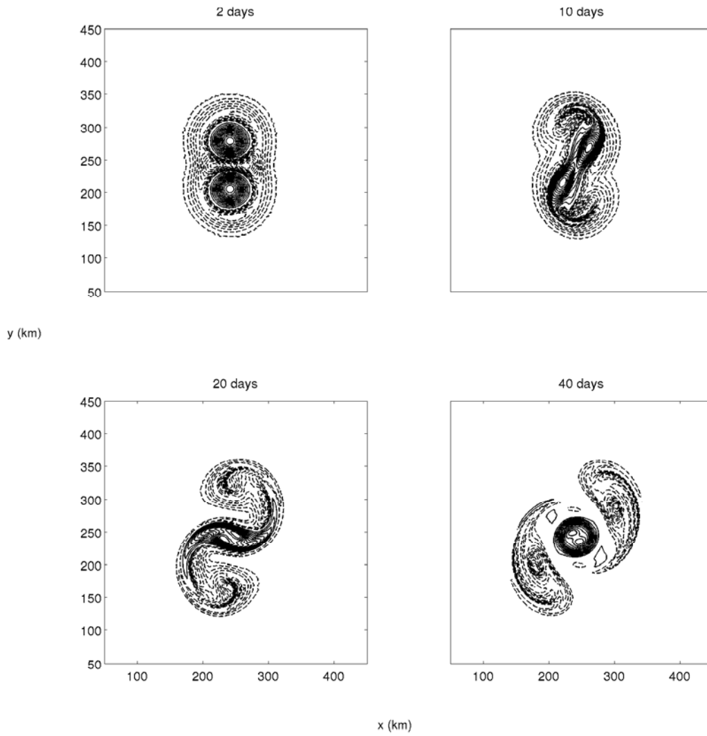
Figure 3. Horizontal sections of PVa at the vortex core. The relative initial distance between the subsurface anticyclones is d_{cm} = 2.5R (M-vortices)
