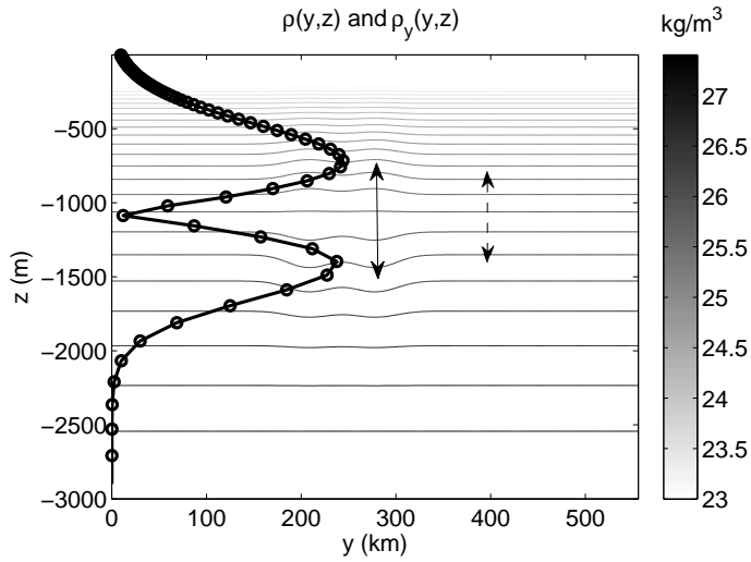
Figure 2. Meridional section of density field \rho(y,z) and its meridional gradient (bold line), in a M case. The solid and dashed arrows indicate the isopycnal deformation induced by the subsurface vortex and the corresponding unperturbed isopycnal layer, respectively.
