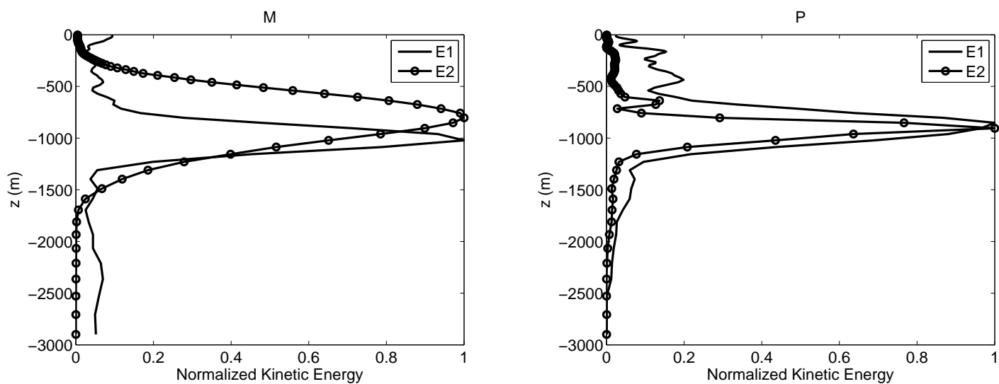
Figure 12. Vertical profiles of kinetic energy through the centers of the eddies E1 and E2 (see also figure 14). Results are presented for M and P-Vortices.
