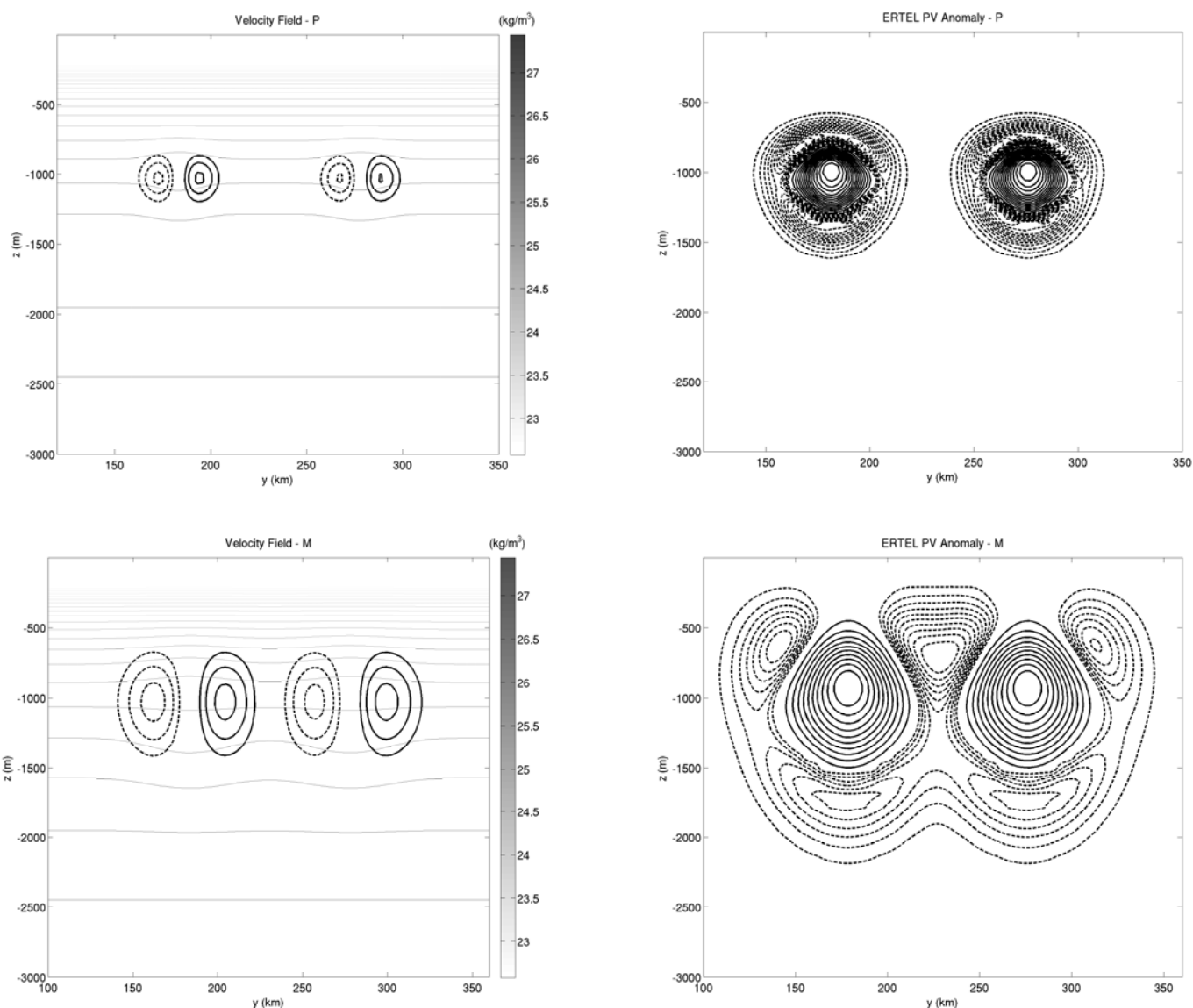
Figure 1. Initial state for subsurface vortex merger experiments with the ROMS model. Top-left and bottom-left: Vertical sections of density and swirl velocity field for P and M-vortices. The bold contours indicate the zonal component of the swirl velocity and go from 0.1 m/s to 0.2 m/s at intervals of 0.05 m/s. Dashed and continuous lines indicate a flow directed towards or going out of the y - z plane, respectively. Top-right and bottom-right: Vertical section of PVa for P and M-vortices. The PVa shields are given by dashed contours.
