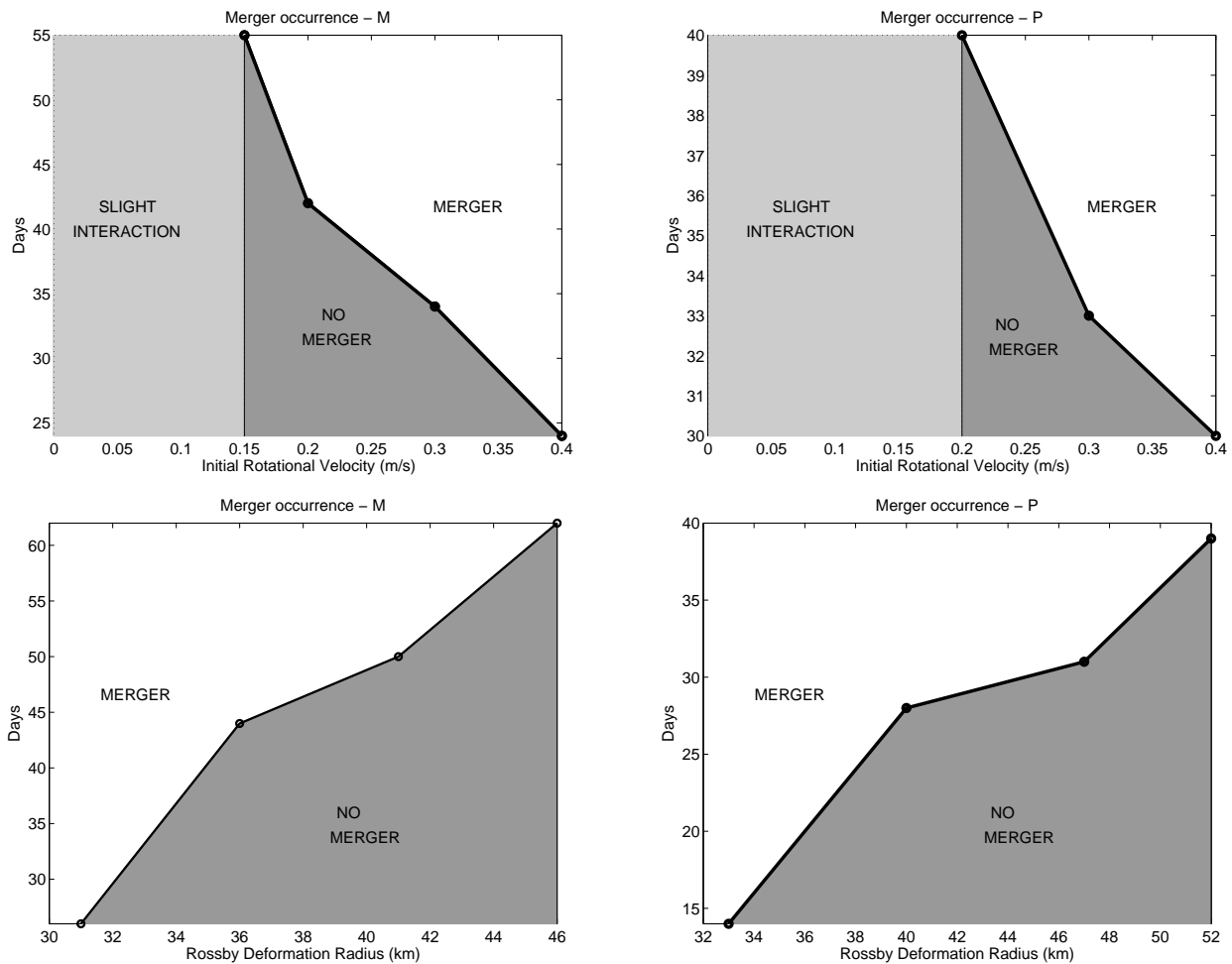
Figure 7. Time required for subsurface vortex merger. Top-left and top-right images show the dependence on initial rotational velocity in a M and P case, respectively. Analogously, bottom-left and bottom-right images show the dependence on the Rossby deformation radius. In the figure, the dots correspond to the experiments actually run in our study.
