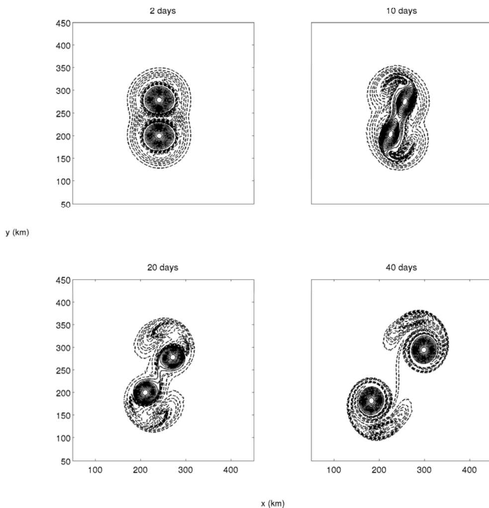
Figure 4. Horizontal sections of PVa at the vortex core. The relative initial distance between the subsurface anticyclones is d = 2.6R (M-vortices)
