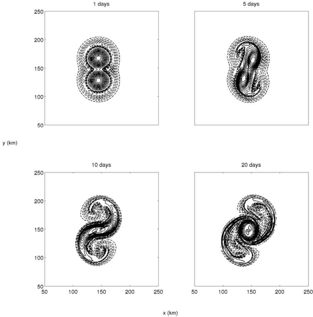
Figure 5. Horizontal sections of PVa at the vortex core. The relative initial distance between the subsurface anticyclones is d = 2.6R (P-vortices)
