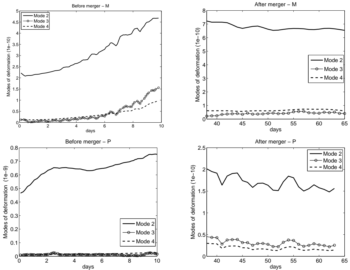
Figure 11. Deformation modes for the subsurface vortex merger. Top-left and top-right figures are related to M-vortices, before and after the merger, respectively. Results for P-vortices are shown in the bottom-left and bottom-right figures.
