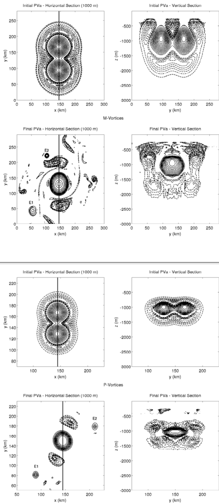
Figure 14. Initial and final sections of PVa for merger of subsurface anticyclones (M and P-Vortices). The vertical sections are estimated along the radial indicated by the bold vertical line. The peripheral eddies are labelled as E1 and E2 in both cases.
