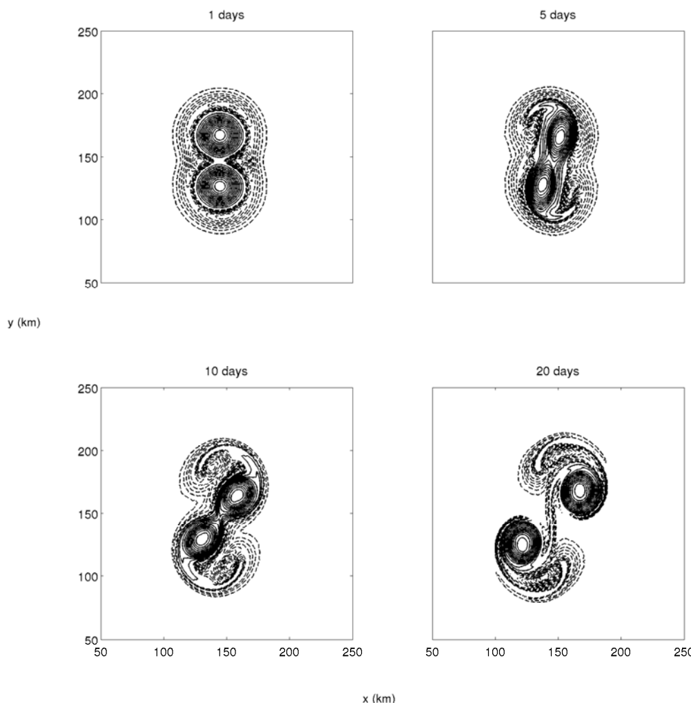
Figure 6. Horizontal sections of PVa at the vortex core. The relative initial distance between the subsurface anticyclones is d = 2.7R (P-vortices)
