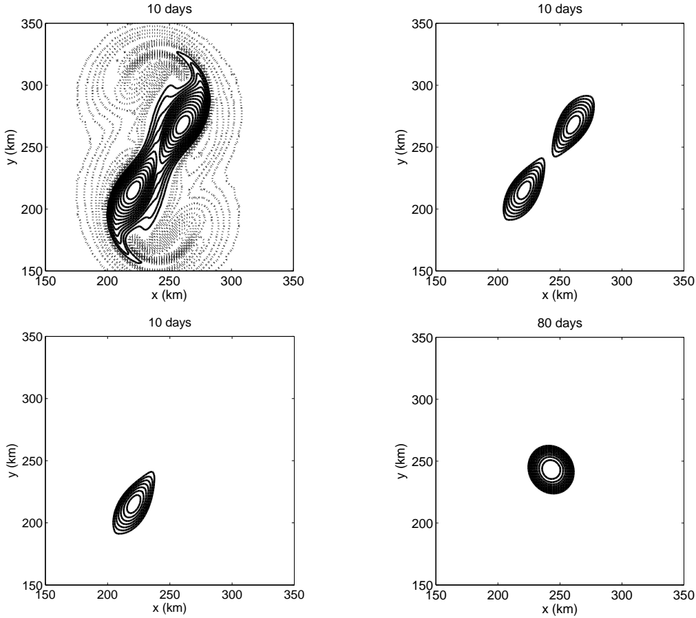
Figure 10. Isolation of a single subsurface vortex for evaluation of the geometric moment. The images show a snapshot of PVa for two M anticyclones during merger (10 days) and after merger (80 days)
