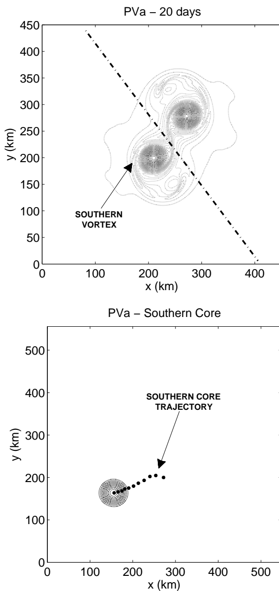
Figure 8. Tracking of a single subsurface vortex for evaluation of the PVa volume integral in the slight interaction case. Top: separation line between the two vortices (dash-dotted line), Bottom: trajectory of the PVa negative core.
