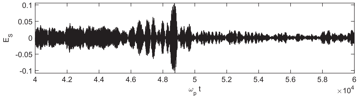
Figure 18. Langmuir waveform (registered electric field E_S as a function of time in arbitrary units) that would be observed by a satellite moving at a velocity v_S = 0.15v_T and starting at a position z_S = 7000\lambda_D at time \omega_p t = 40000 ; the satellite travels until the time \omega_p t = 60000 . The parameters are the same as in Figure 12, but with \Delta n \simeq 0.03 .
