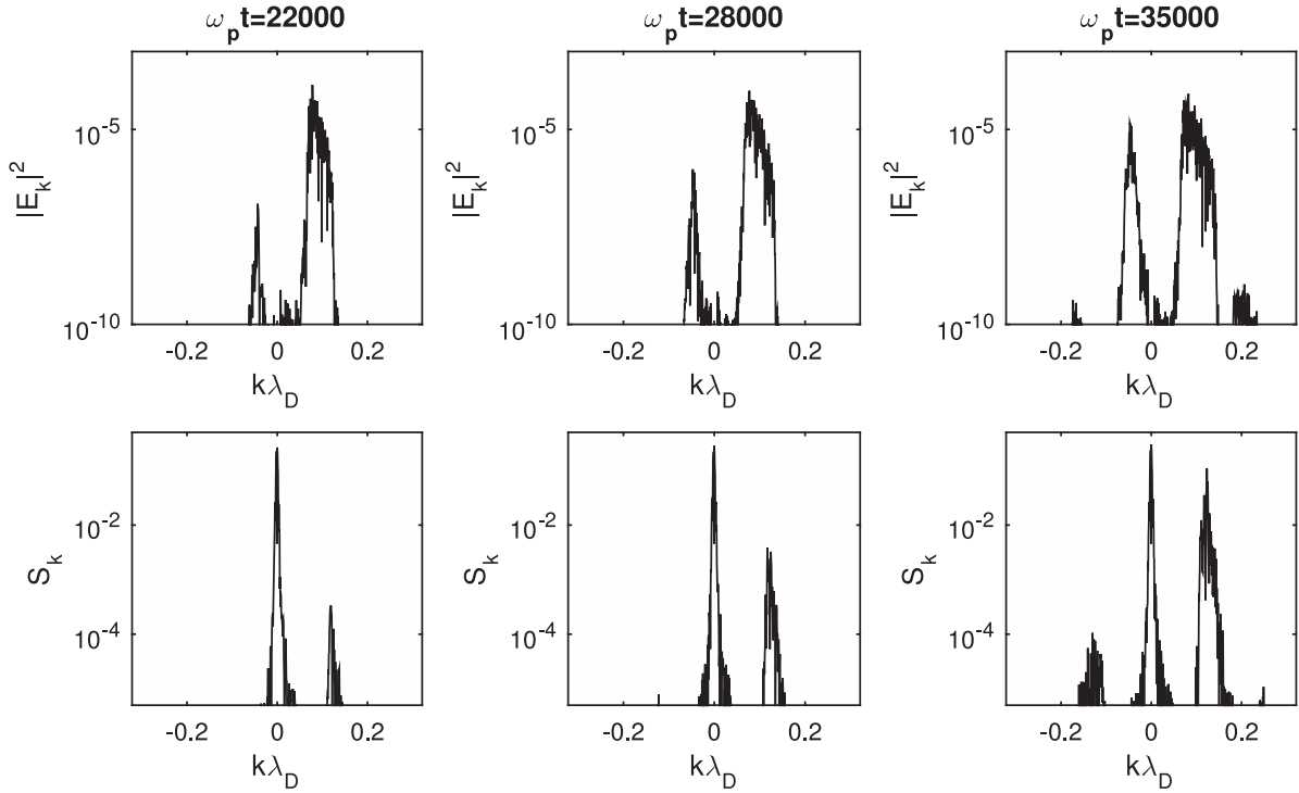
Figure 4. Upper panels: spectra |E_k|^2 of the Langmuir waves (in logarithmic scales) for the same instants of time as in Figure 2, i.e., \omega_p t = 22000, 28000, and 35000 , as a function of k\lambda_D . Lower panels: Corresponding spectra (in logarithmic scales) of the energy density S_k of the IS waves with k \geq 0 propagating in the positive direction and of the IS waves with k < 0 propagating in the negative direction. Parameters are the same as in Figure 1.
