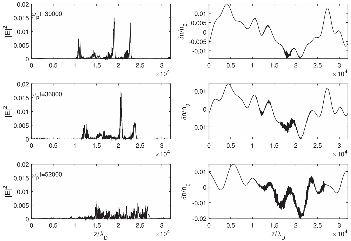
Figure 7. Left panels: profiles of the Langmuir wave energy |E|^2 (turbulence parameter) at times \omega_p t = 30000 , 36000 , and 52000 . Right panels: corresponding profiles of the density fluctuations \delta n/n_0 . The space coordinate z/\lambda_D ranges from 0 to the size L of the simulation box. The parameters are the same as in Figure 6.
